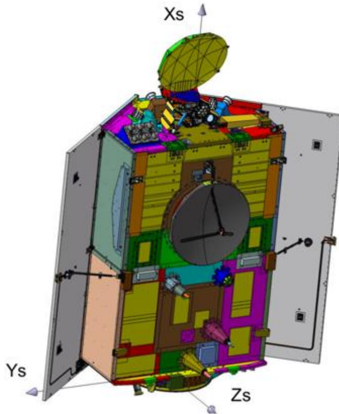
Figure 2-2 Satellite Reference frame definition origin is located at the interface plane separating the launcher and the satellite.
