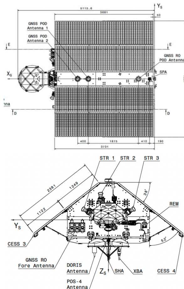
Figure 2-4 Deployed solar array area.
