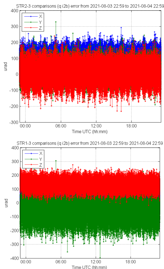
Figure 2-11 Angular offset in body frame between all STRs in eclipse-free Normal Mode Attitude Hold. The assessment shown is during daylight only using the on-board body-alignment quaternions pertaining to the day-night average.
