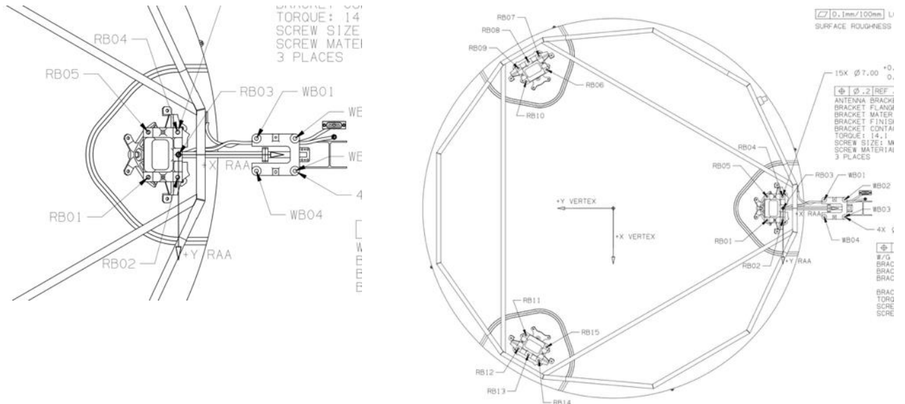
Figure 2-8 (Left) Poseidon-4 instrument reference (RAA) frame definition , which is by design orthogonal with the satellite reference frame (see Figure 2-7), though in practice has a small rotation since physically it is linked with the assembly of an instrument panel onto the satellite structure. (Right) RF measurements have been defined in an antenna reference (vertex) frame for RF measurements, though all analysed measurements provided in this section have been translated from this frame to the RAA and the SRF.
