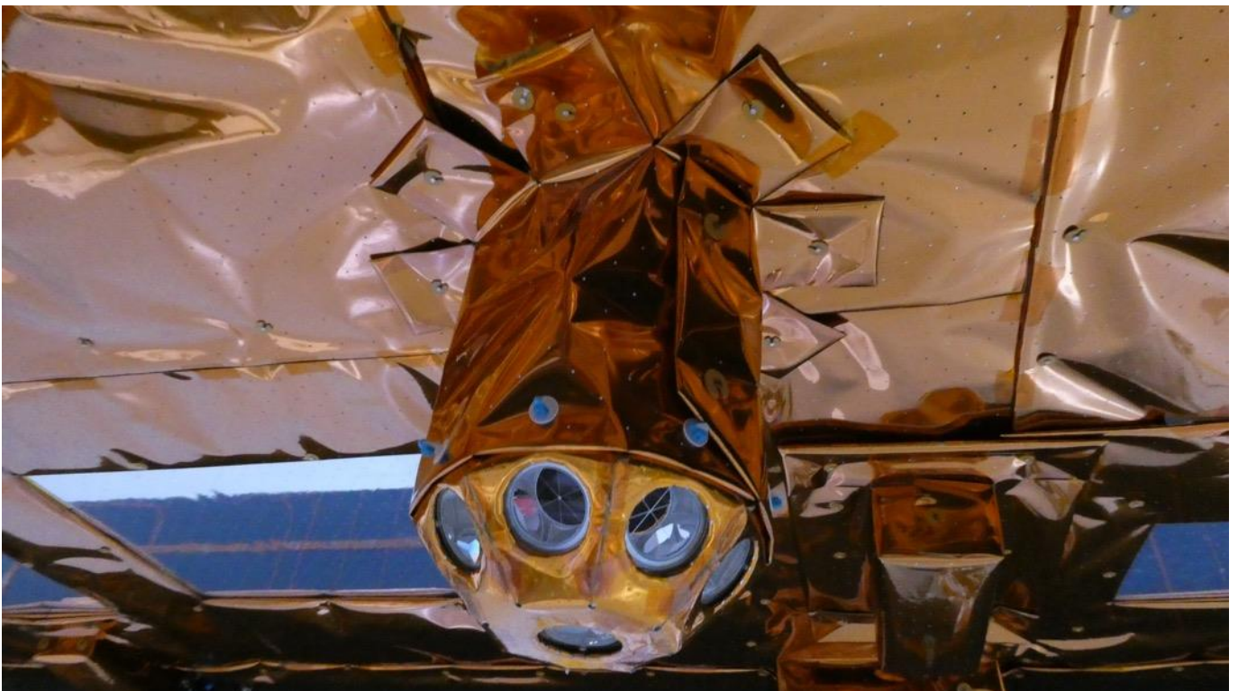
Figure 4-17 Laser Retro-Reflector
