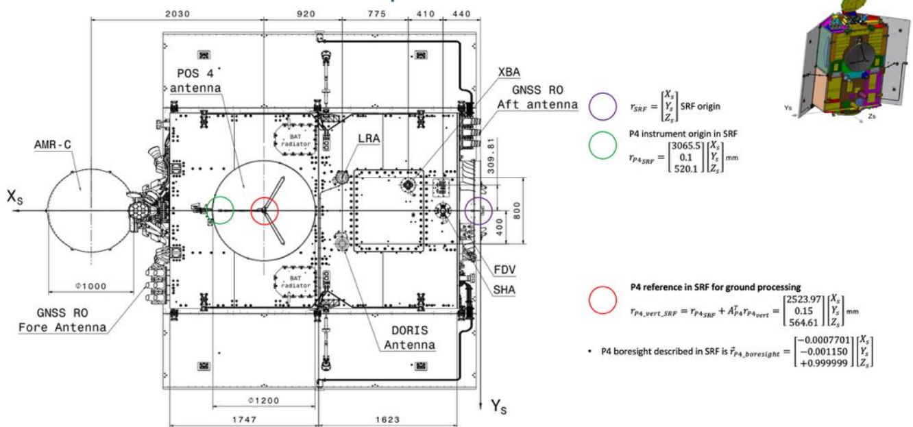
Figure 2-7 The Satellite Reference Frame definition with the key reference points of the Poseidon-4 viewing from underneath the satellite.
