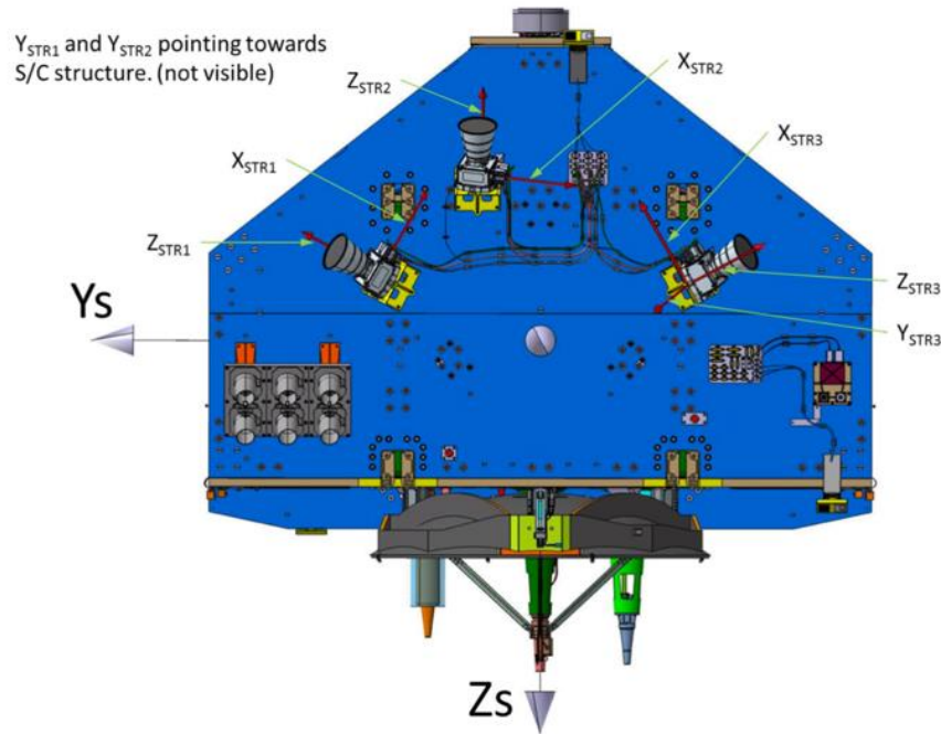
Figure 2-10 Location of the three star tracker camera heads and baffles.
