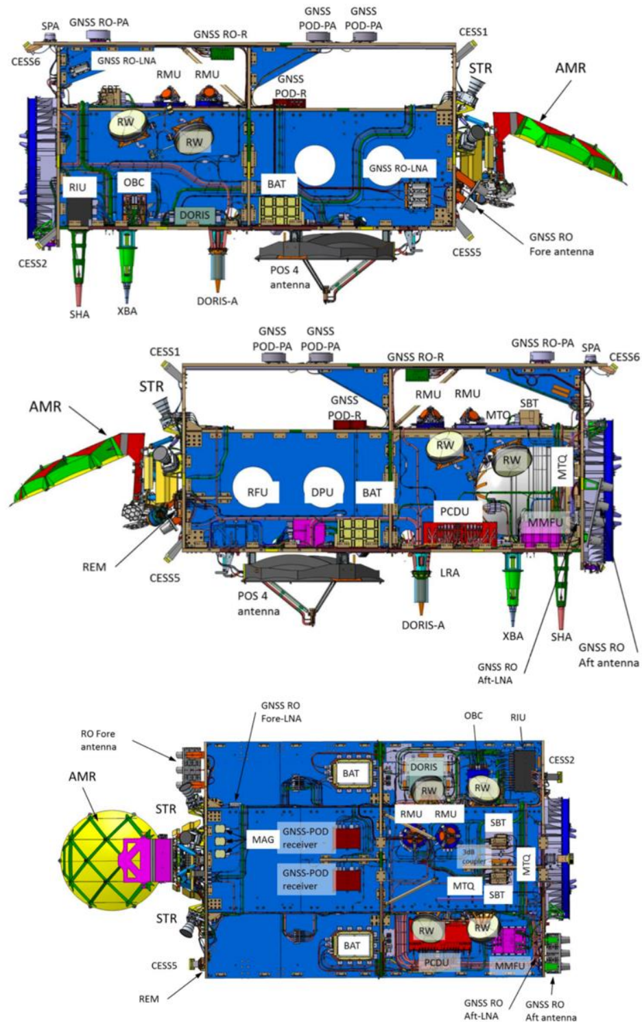
Figure 2-1 With reference to the definition of the spacecraft axes, Figure 2-2. (Top) Spacecraft looking along the +Y axis, (Middle) looking along the -Y axis and (Bottom) looking along the -Z axis.
