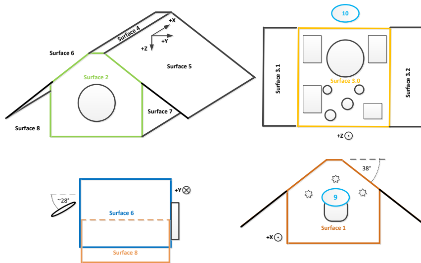
Figure 2-3 The 12 panel model for which properties are provided in §2.4.1
