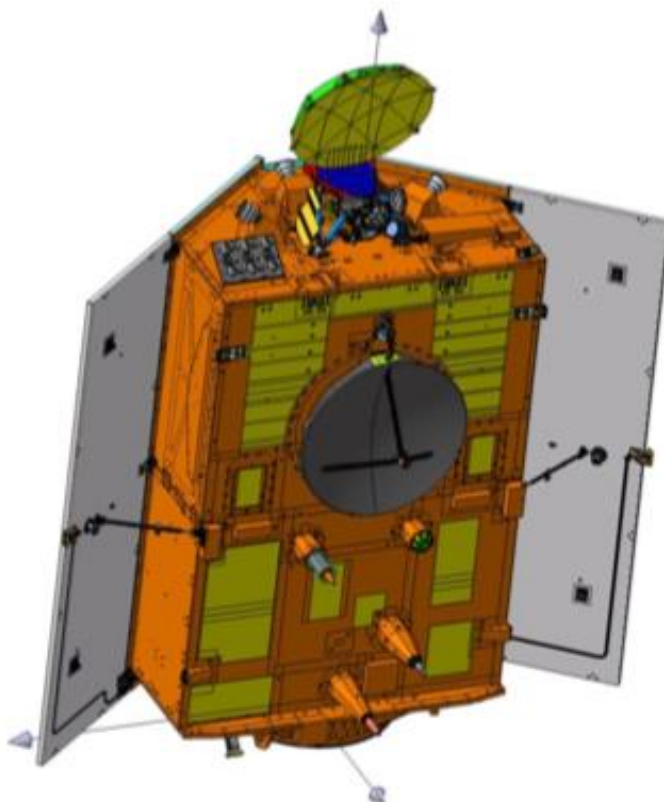
Figure 2-5 MLI covering in orange, SSM in yellow and CFRP in grey.
