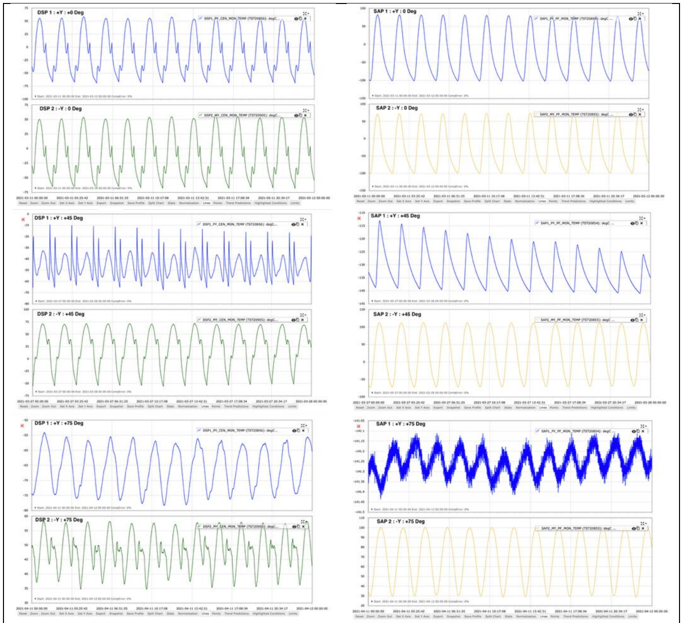
Figure 2-6 DSP (Left) and SAP (Right) thermistor plots at (from top to bottom) approximately -80°, -45°, 0°, +45° and +75° of solar beta angle. Each of the 12 plots shows the DSP or SAP elements pointing in the +Y (top denoted 1) and -Y (bottom denoted 2).
