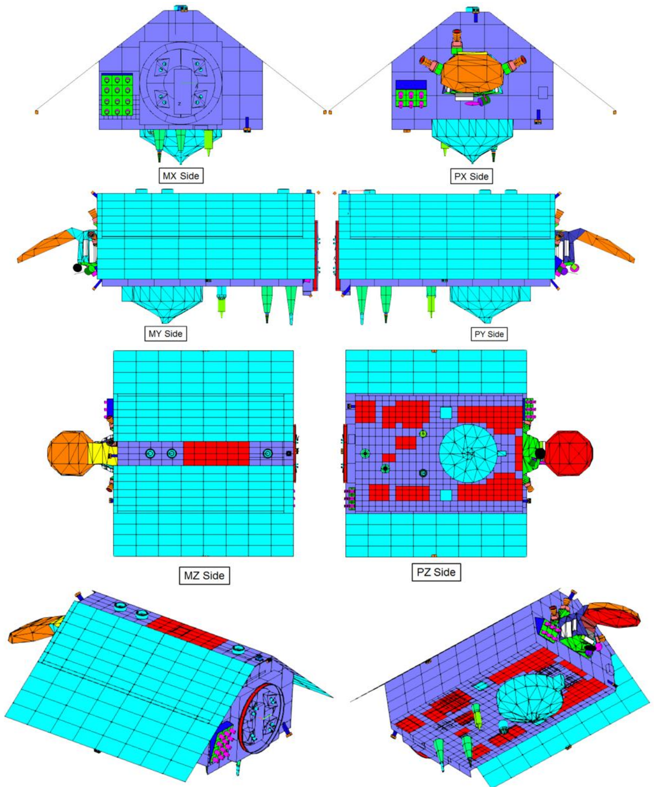
Figure 4-1 Different orientations of the spacecraft with ‘P’ meaning the projection from the positive X, Y or Z axis and ‘M’ from the negative X, Y or Z axis.
