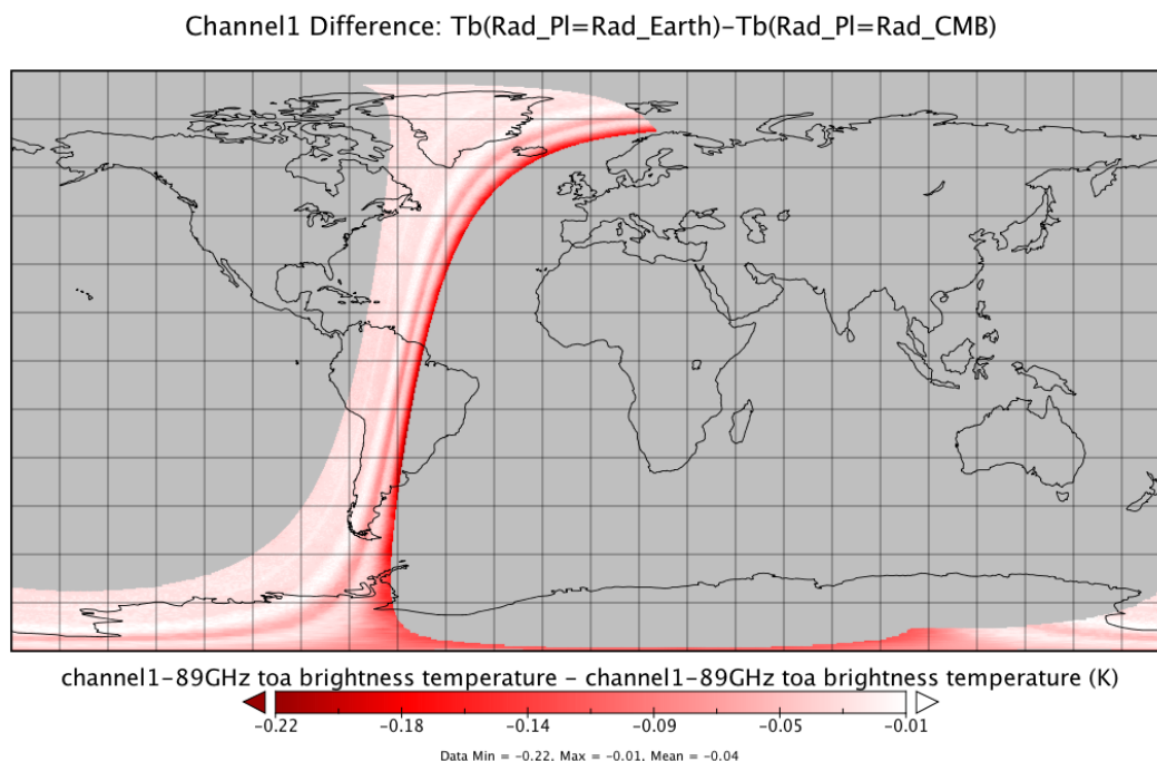
Figure 11 Difference of Earth pixel brightness temperatures from two evaluations of the measurement equation: 1. Evaluation follows the assumption made in AAPP, i.e. radiance of Platform = Radiance of Earth”, 2. Evaluation assumes “radiance of Platform =Radiance of Cold Space”. This figure shows the result for Channel1 1. Maximum difference of the evaluations is -0.22 K at the edge of the swath.
