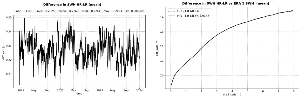
Figure 67: HR-LR MLE4 difference for Ku-band SWH. Left: mean per day. Right: difference with respect to ERA5 SWH, computed on the entire time series (dotted line) and on 2023 only (solid line).
