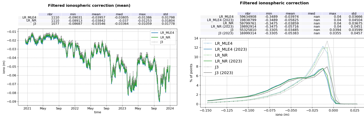
Figure 82: Monitoring of filtered ionospheric correction for Sentinel-6 MF LR MLE4 (blue), LR NR (green) and Jason-3 (black). Left: Mean per day. Right: Histogram computed on the entire time series (dotted line) and on 2023 only (solid line).
