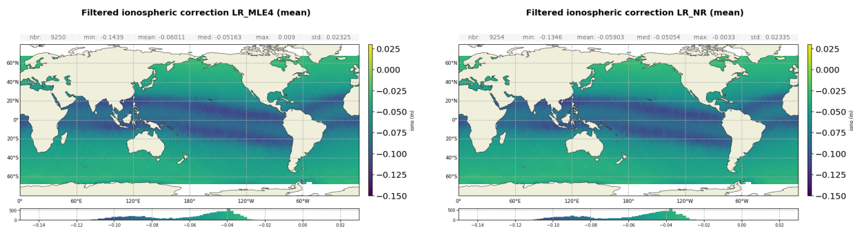
Figure 83: Maps of mean filtered ionospheric correction for Sentinel-6 MF LR MLE4 (left) and LR NR (right). Computed on year 2023.
