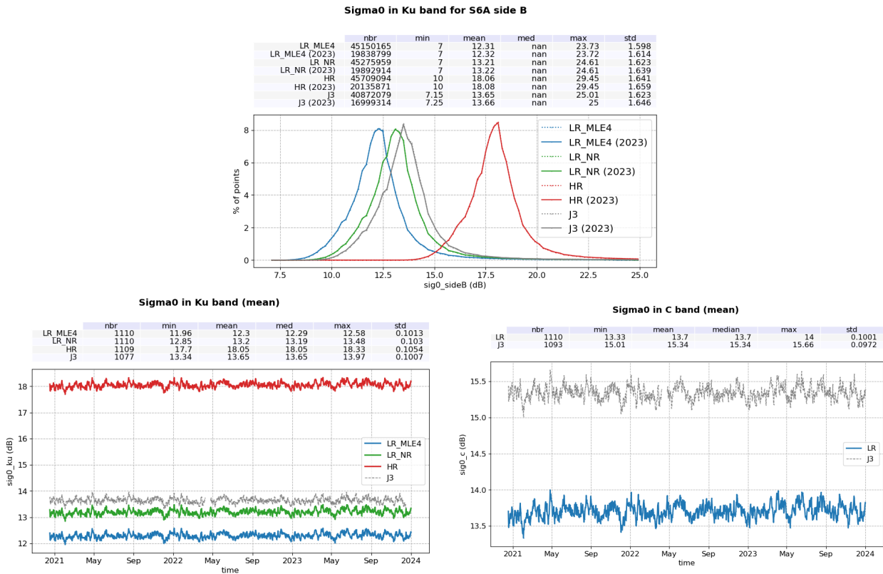
Figure 68: Top : Histogram of Ku-band Sigma0 for Sentinel-6 MF LR MLE4 (blue), LR NR (green), Sentinel-6 MF HR (red) and Jason-3 (black), computed on POS4-B entire time period (dotted line) and on 2023 only (solid line). Bottom: daily monitoring of Sigma0 mean in Ku-band (left) and C-band (right).
