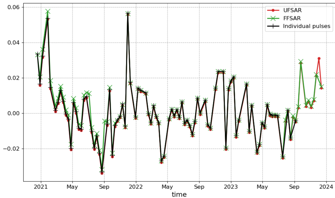
Figure 99: Monitoring of the range bias at CDN1 transponder, from cycle 34 to 115.
