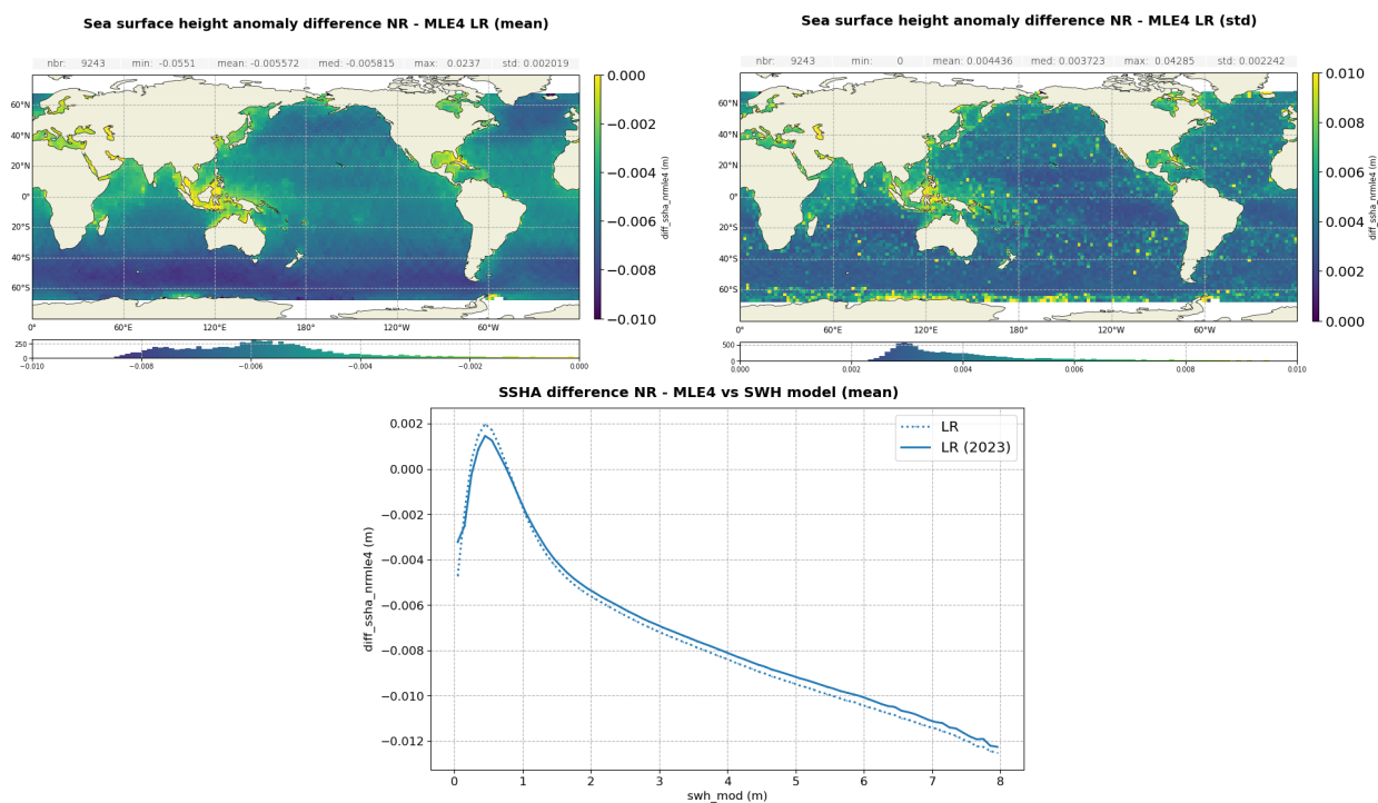
Figure 105: Maps of mean ( left ) and standard deviation ( right ) of Sentinel-6 MF LR NR - MLE4 SSHA in meters, and its mean as a function of ERA 5 model SWH ( bottom ).
