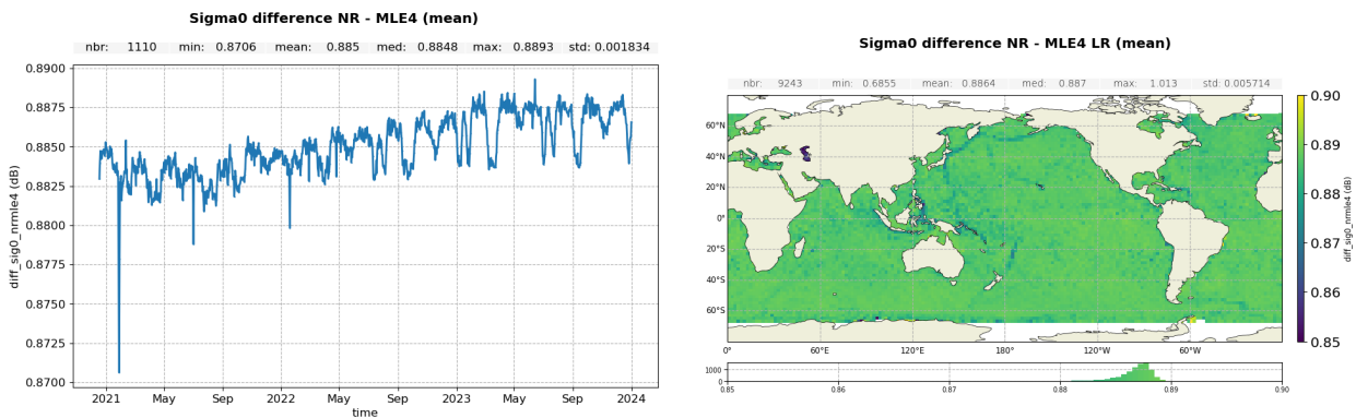
Figure 70: Map (right) and monitoring (left) of the LR NR - MLE4 sigma0 difference per day.
