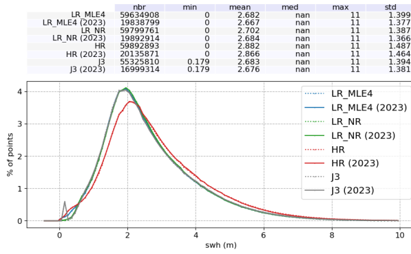
SWH in Ku band (mean)
