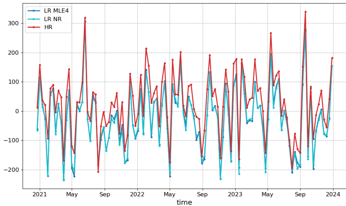
Figure 100: Monitoring of the datation bias at CDN1 transponder, from cycle 34 to 115.
