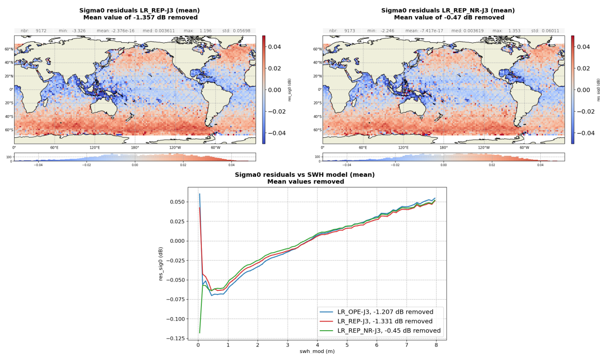
Figure 80 – Ku-band backscatter coefficient difference: Sentinel-6 MF LR minus Jason-3 computed over the complete tandem period. Gridded map for reprocessed MLE4 ( left ) and NR ( right ) and difference function of ERA 5 model SWH ( bottom ).
