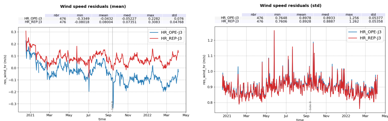
Figure 94 – Time monitoring of Ku-band wind speed difference: Sentinel-6 MF HR minus Jason-3. Mean per day ( left ) and standard deviation per day ( right ) computed over the complete tandem period for operational (blue) and reprocessed (red) datasets.
