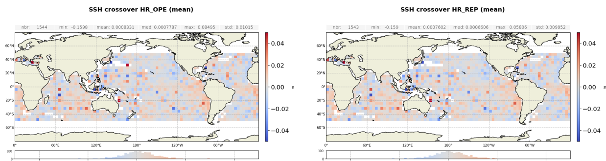
Figure 69 – Mean SSH difference at crossovers for Sentinel-6 MF HR operational data ( left ) and reprocessed data ( right ). Computed over the complete reprocessing period.
