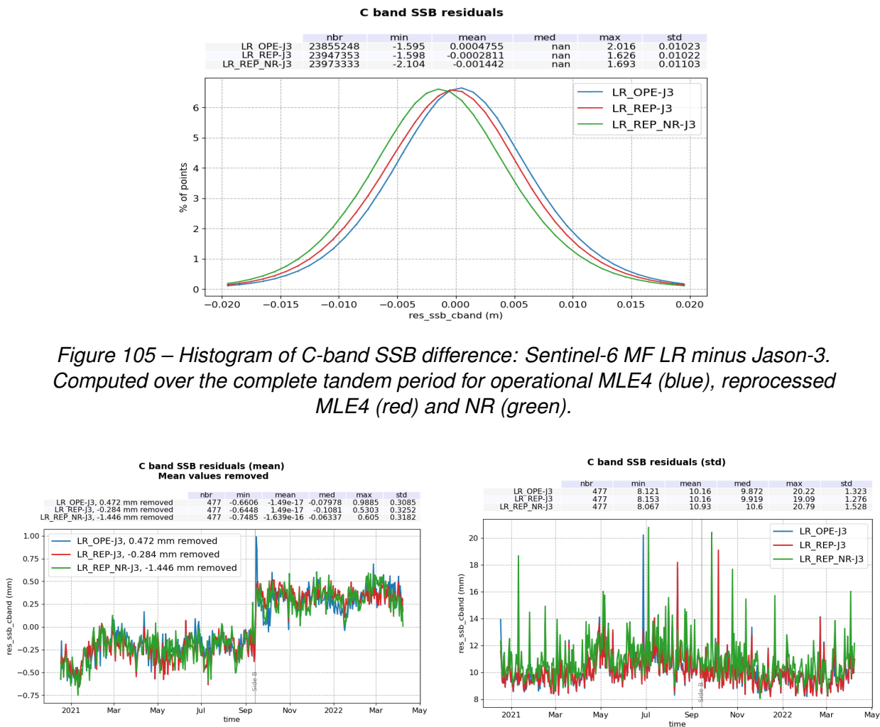
Figure 106 – Time monitoring of C-band SSB difference: Sentinel-6 MF LR minus Jason-3. Mean per day (left) and standard deviation per day (right) computed over the complete tandem period for operational MLE4 (blue), reprocessed MLE4 (red) and NR (green).
