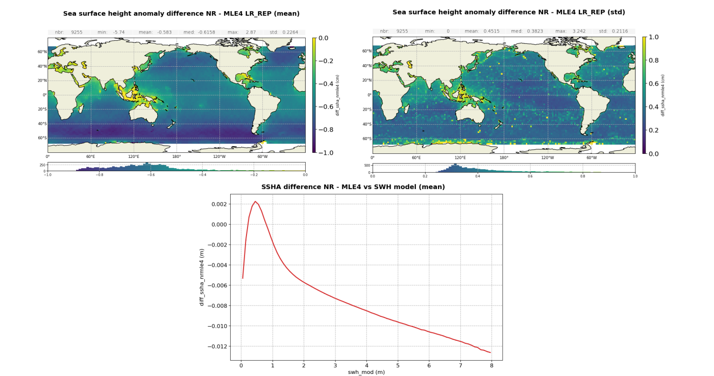
Figure 62 – Maps of mean ( left ) and standard deviation ( right ) of Sentinel-6 MF LR reprocessed NR - MLE4 SSHA in meters, and its mean as a function of ERA 5 model SWH ( bottom ).
