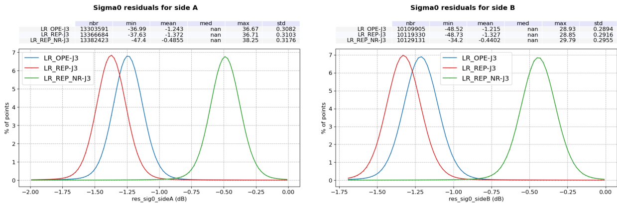
Figure 78 – Histogram of Ku-band backscatter coefficient difference: Sentinel-6 MF LR minus Jason-3. Computed over POS-4 side A (left) and side B (right) periods, for operational MLE4 (blue), reprocessed MLE4 (red) and NR (green).
