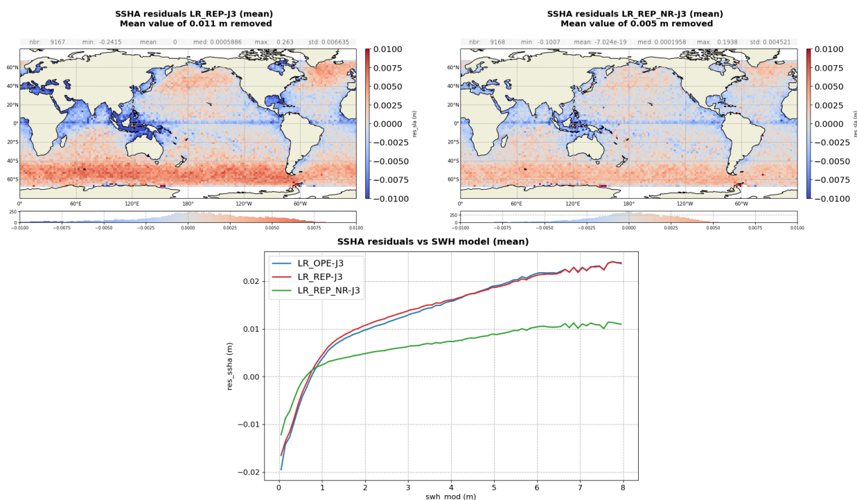
Figure 114 – SSHA difference: Sentinel-6 MF LR minus Jason-3 computed over the complete tandem period. Gridded map for reprocessed MLE4 ( left ) and NR ( right ) and difference function of ERA 5 model SWH ( bottom ).
