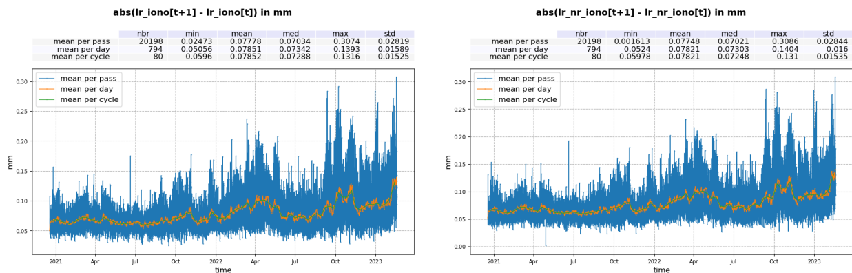
Figure 125 – Absolute value of consecutive filtered ionosphere correction measurement for MLE4 (left) and NR (right). Mean per pass (blue), mean per day (orange) and mean per cycle (green).
