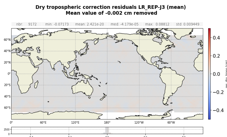
Figure 130 – Mean gridded map of dry tropospheric correction difference: Sentinel-6 MF LR minus Jason-3. Computed over cycles 4 to 51.
