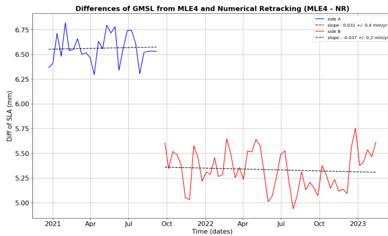
Figure 122 – GMSL difference MLE4 - NR SLAs over the reprocessed period. Slope errors are given at 90 % C.L.
