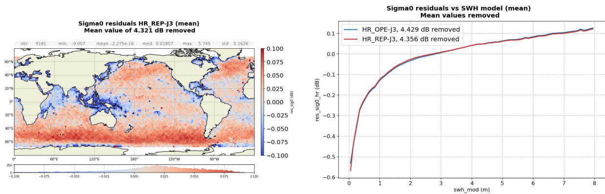
Figure 92 – Ku-band backscatter coefficient difference: Sentinel-6 MF HR minus Jason-3 computed over the complete tandem period. Gridded map for reprocessed dataset ( left ) and difference function of ERA 5 model SWH ( right ).
