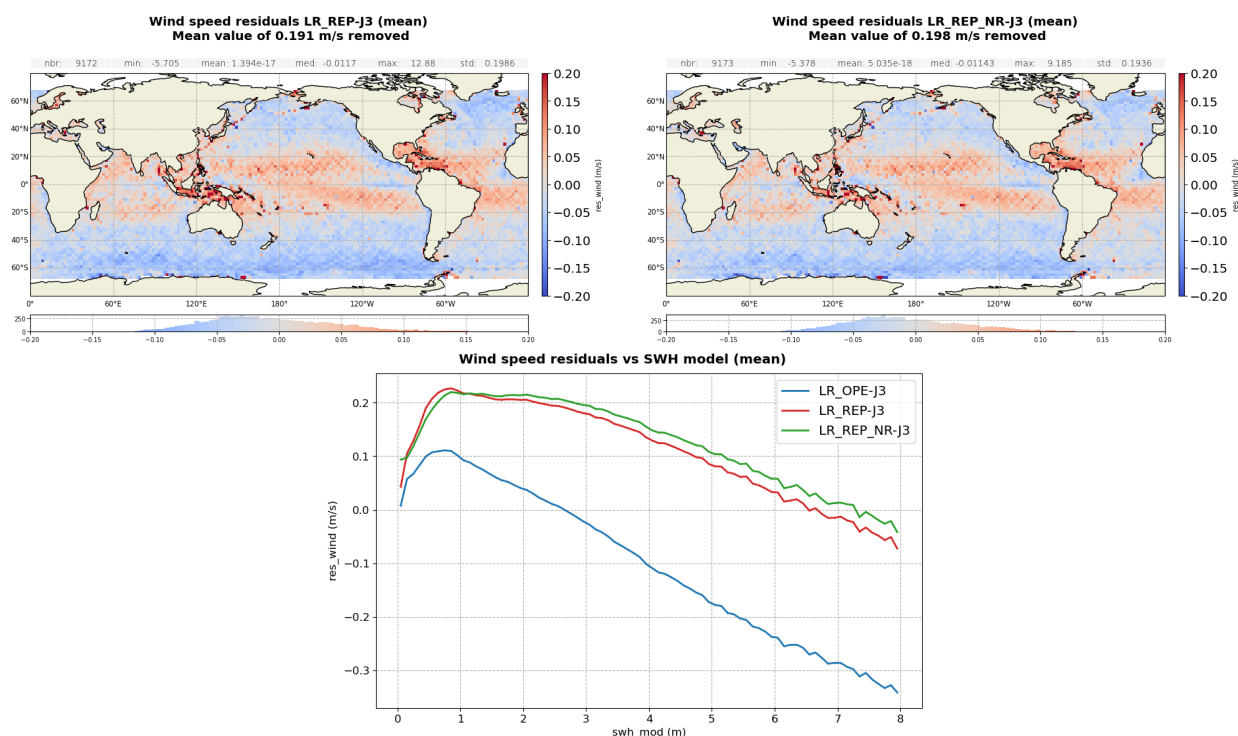
Figure 83 – Altimeter wind speed difference: Sentinel-6 MF LR minus Jason-3 computed over the complete tandem period in m/s. Gridded map for reprocessed MLE4 ( left ) and NR ( right ) and difference function of ERA 5 model SWH ( bottom ).
