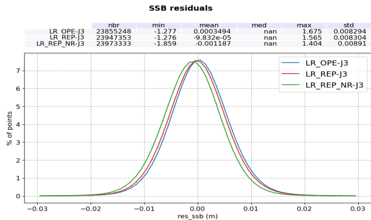
Figure 84 – Histogram of Ku-band SSB difference: Sentinel-6 MF LR minus Jason-3. Computed over the complete tandem period for operational MLE4 (blue), reprocessed MLE4 (red) and NR (green).
