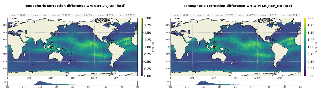
Figure 127 – Standard deviation gridded map of the difference between Altimeter Filtered Ionosphere correction and GIM model (cm) for MLE4 ( left ) and NR ( right ). Computed over the entire reprocessing period.
