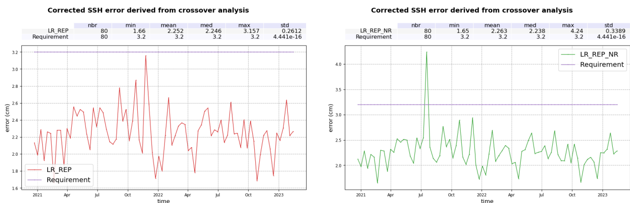
Figure 133 – Corrected LR SSH error derived from crossover analysis with a selection over Pacific patch (latitude in [-24.5°N; -3°N] and longitude in [220°E; 246°E]), in cm for MLE4 (left) and for NR (right). The error equals to the standard deviation of the SSH difference divided by \sqrt{2} . Computed on a cyclic basis.
