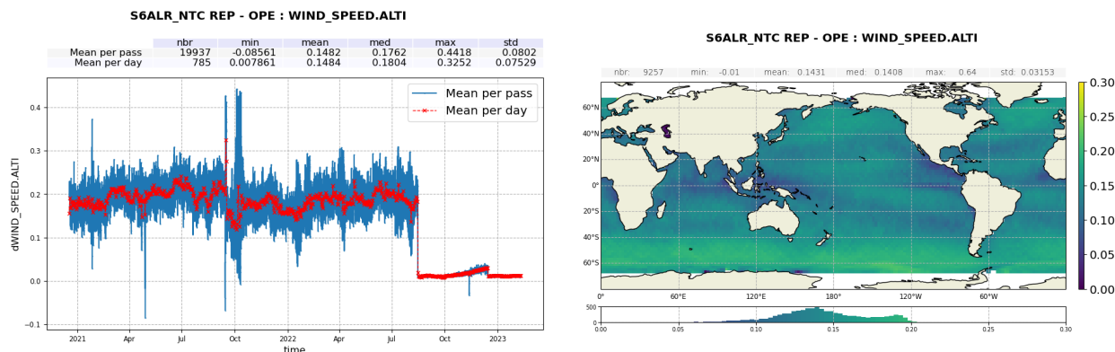
Figure 32 – Map ( right ) and monitoring ( left ) of the LR MLE4 operational - reprocessed wind speed difference per day (red) and per pass (blue).
