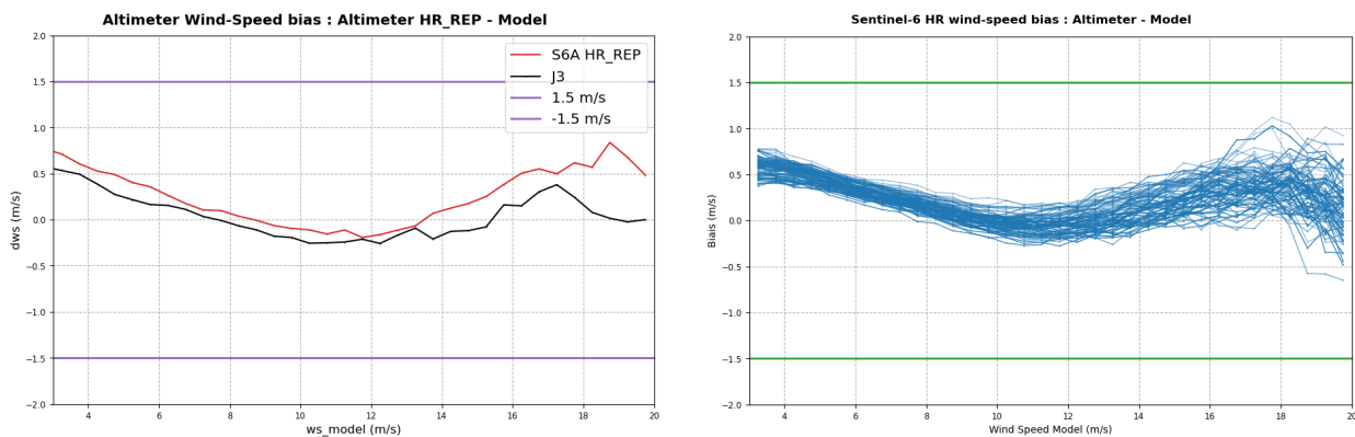
Figure 143 – Difference between Altimeter HR wind speed and model wind speed function of model wind speed, in m/s. Computed over Sentinel-6 MF cycle 70 (left) and for all cycles (right, darker curves correspond to more recent cycles). Green lines represent requirement limits.
