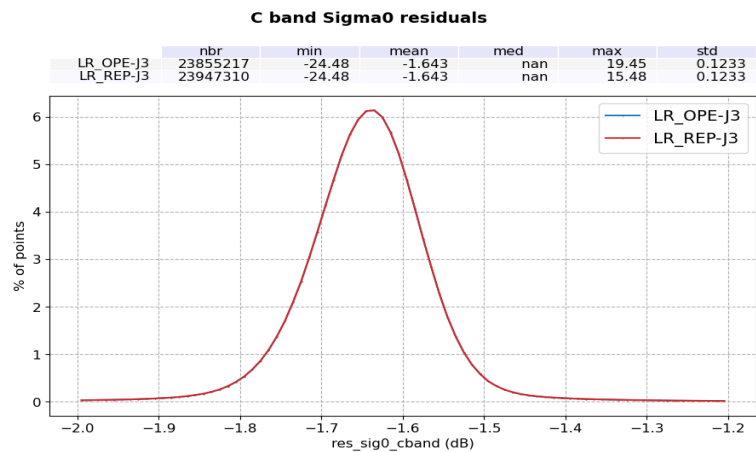
Figure 102 – Histogram of C-band backscatter coefficient difference: Sentinel-6 MF LR minus Jason-3. Computed over the complete tandem period, for the operational (blue) and reprocessed (red) datasets.
