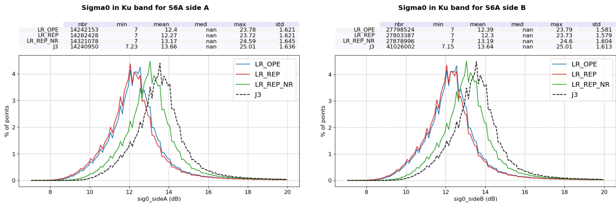
Figure 24 – Histogram of Sentinel-6 MF LR Ku-band Backscatter coefficient in dB, before reprocessing (blue) and after reprocessing (red for MLE4 and green for NR) and Jason-3 (black), for side A (left) and side B (right).
