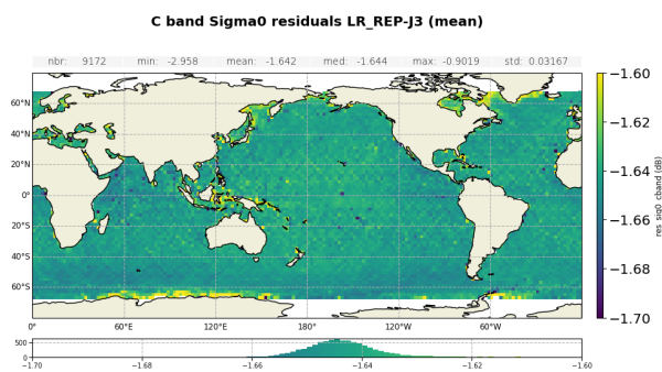
Figure 104 – C-band backscatter coefficient difference: Sentinel-6 MF reprocessed LR minus Jason-3 computed over the complete tandem period. Gridded map ( left ) and difference function of ERA 5 model SWH ( right ).
