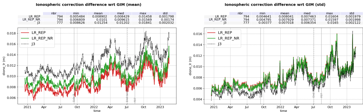
Figure 47 – Time monitoring of the ionosphere correction difference : Altimeter Filtered minus GIM model (m), for Jason-3 (black) and Sentinel-6 MF LR reprocessed data (red for MLE4, green for NR). Left : mean per day, right : standard deviation per day.
