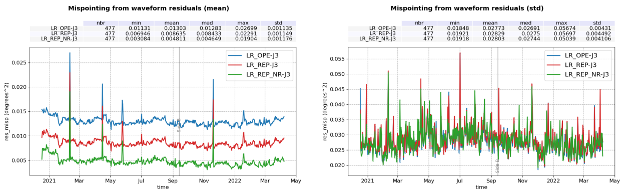
Figure 88 – Time monitoring of mispointing difference: Sentinel-6 MF LR minus Jason-3. Mean per day ( left ) and standard deviation per day ( right ) computed over the complete tandem period for operational MLE4 (blue), reprocessed MLE4 (red) and NR (green).
