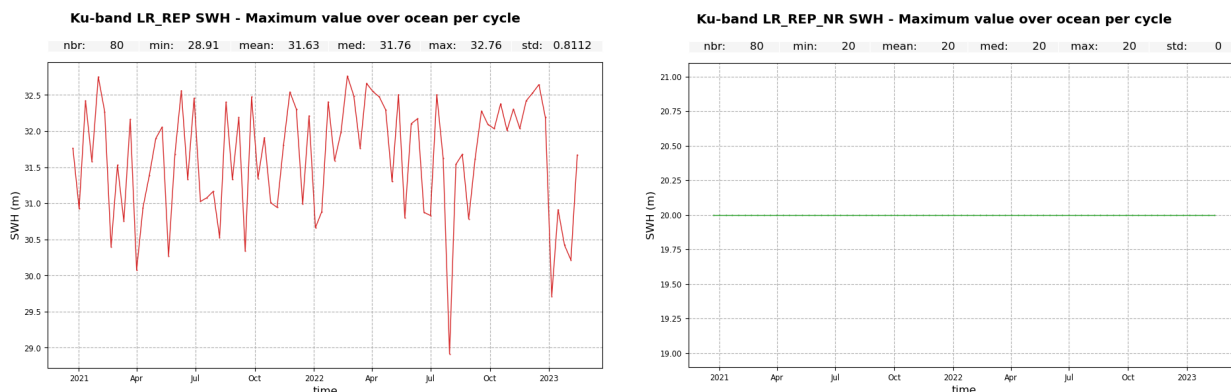
Figure 135 – Maximum value of Sentinel-6 MF LR SWH per cycle for MLE4 ( left ) and NR ( right ).
