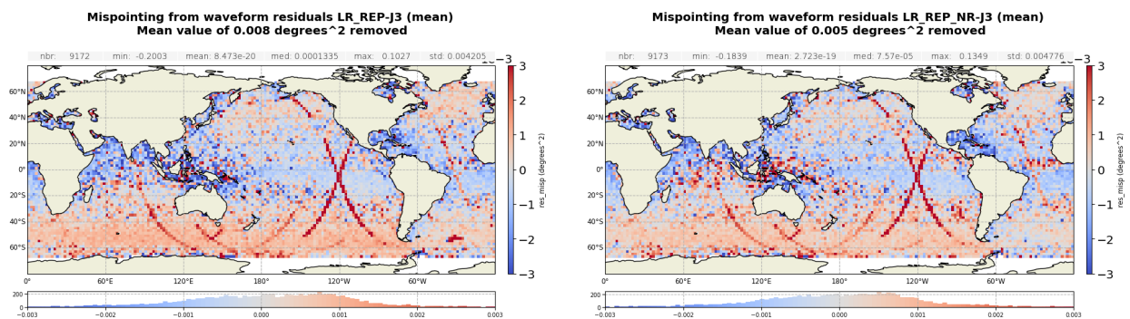
Figure 89 – Mispointing difference: Sentinel-6 MF LR minus Jason-3 computed over the complete tandem period. Gridded map for reprocessed MLE4 ( left ) and NR ( right ).
