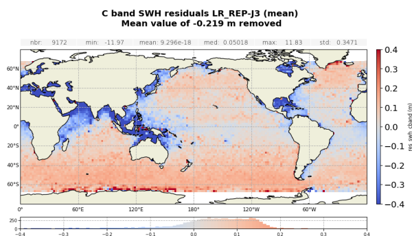
Figure 98 – C-band SWH difference: Sentinel-6 MF LR minus Jason-3 computed over the complete tandem period. Gridded map for the reprocessed dataset ( left ) and difference function of ERA5 SWH ( right ).
