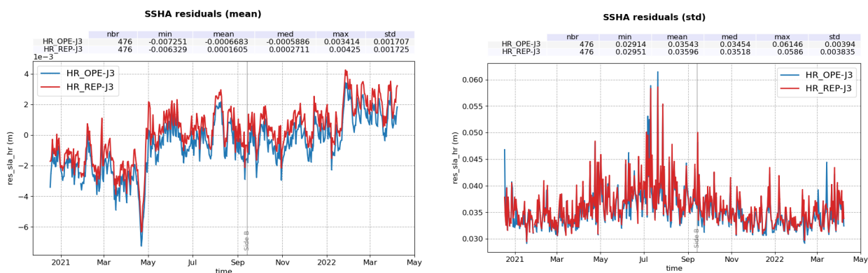
Figure 116 – Time monitoring of product SSHA difference: Sentinel-6 MF HR minus Jason-3. Mean ( left ) and standard deviation ( right ) per day computed over the complete tandem period for operational and reprocessed (red) datasets.
