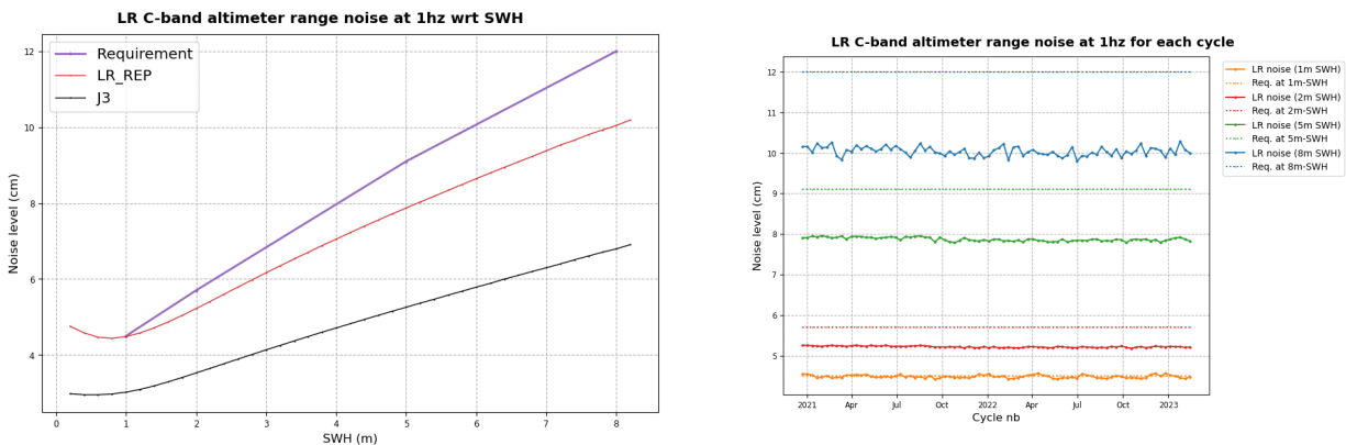
Figure 124 – 1 Hz noise of LR C-band altimeter range. Left panel: noise function of SWH for Sentinel-6 MF LR and Jason-3; the purple line represents the requirement thresholds. Right panel : noise level computed for each cycle and at 1, 2, 5 and 8 m-wave (solid lines) and the corresponding requirement levels (dashed lines).
