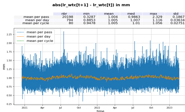
Figure 131 – Absolute value of consecutive AMR-C WTC measurement in mm. Mean per pass (blue), mean per day (orange) and mean per cycle (green).
