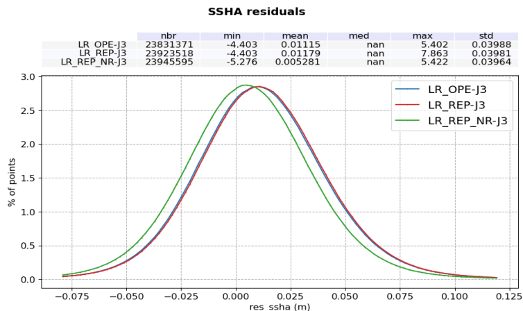
Figure 111 – Histogram of product SSHA difference: Sentinel-6 MF LR minus Jason-3. Computed over the complete tandem period for operational MLE4 (blue), reprocessed MLE4 (red) and NR (green).
