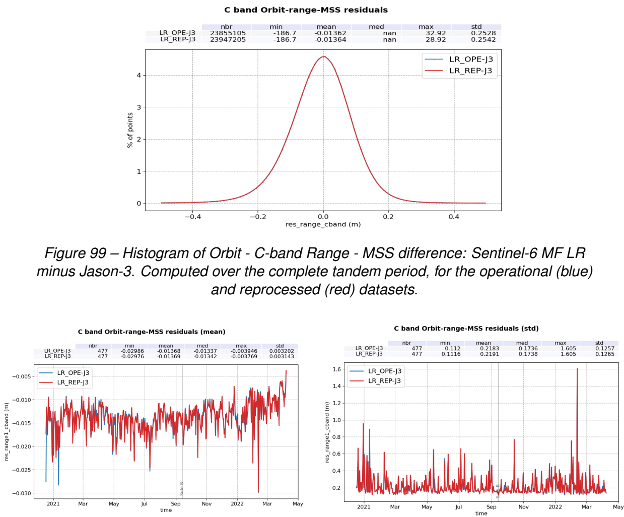
Figure 99 – Histogram of Orbit - C-band Range - MSS difference: Sentinel-6 MF LR minus Jason-3. Computed over the complete tandem period, for the operational (blue) and reprocessed (red) datasets. Figure 100 – Time monitoring of Orbit - C-band Range - MSS difference: Sentinel-6 MF LR minus Jason-3. Mean per day (left) and standard deviation per day (right) computed over the complete tandem period, for the operational (blue) and reprocessed (red) datasets.
