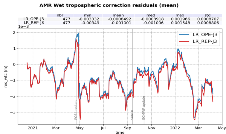
Figure 71 – Time monitoring of Radiometer WTC difference : Sentinel-6 MF AMR-C minus Jason-3 AMR. Mean per day for the operational (blue) and reprocessed (red) datasets, computed over the complete tandem period.
