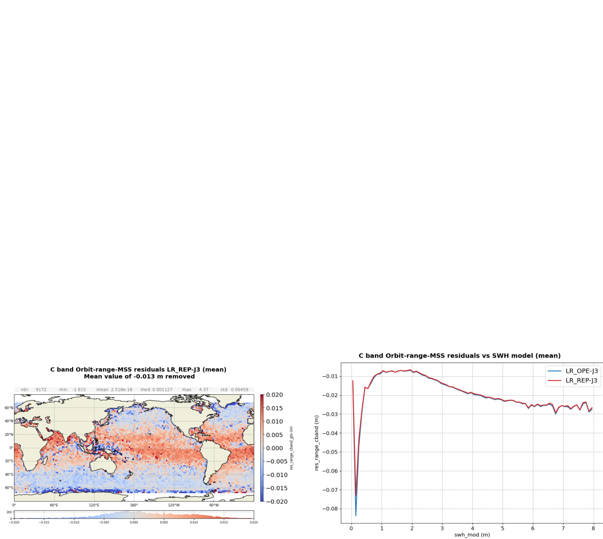
Figure 101 – Orbit - C-band Range - MSS difference: Sentinel-6 MF LR minus Jason-3 computed over the complete tandem period. Gridded map (left panel) and difference function of ERA 5 model SWH (right panel).
