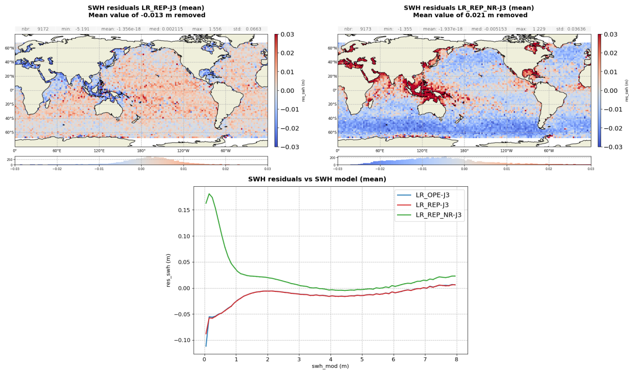
Figure 74 – Ku-band SWH difference: Sentinel-6 MF LR minus Jason-3 computed over the complete tandem period. Gridded maps for S6 MF MLE4 (left) and NR (right), and differences function of ERA 5 model SWH (bottom).
