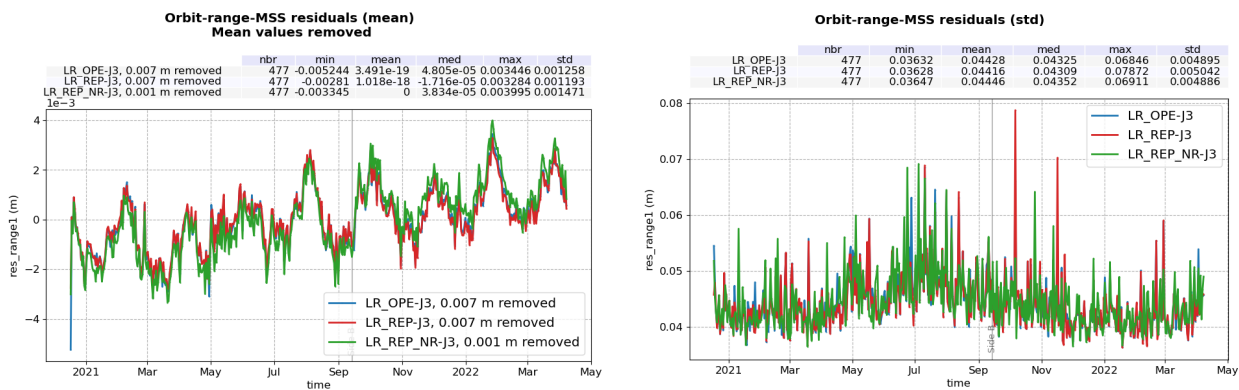
Figure 76 – Time monitoring of Orbit - Ku-band range - MSS difference: Sentinel-6 MF LR minus Jason-3. Mean per day (left) and standard deviation per day (right) computed over the complete tandem period.
