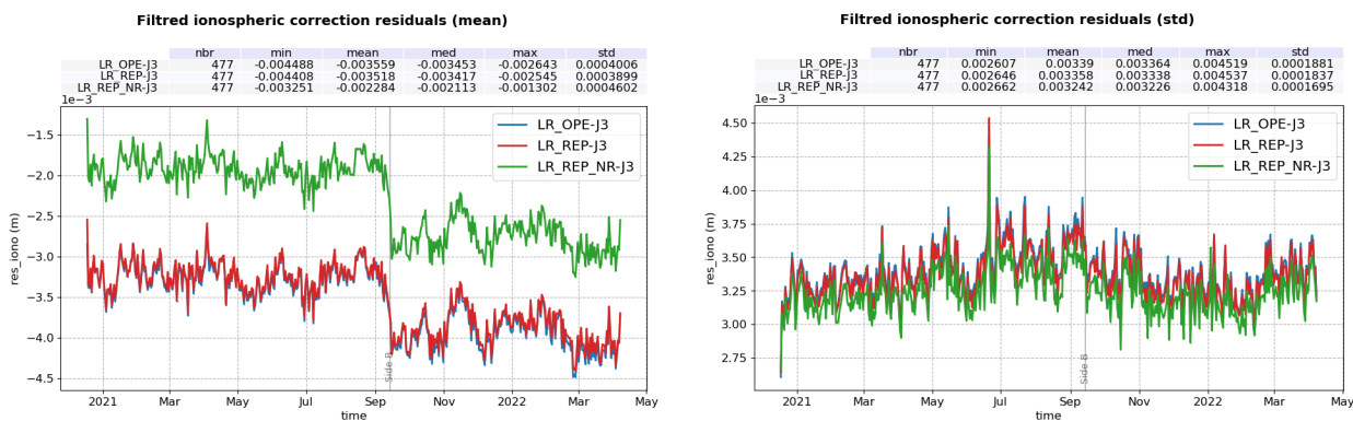
Figure 109 – Time monitoring of Filtered Altimeter Ionosphere correction difference: Sentinel-6 MF LR minus Jason-3. Mean per day (left) and standard deviation per day (right) computed over the complete tandem period for operational MLE4 (blue), reprocessed MLE4 (red) and NR (green).
