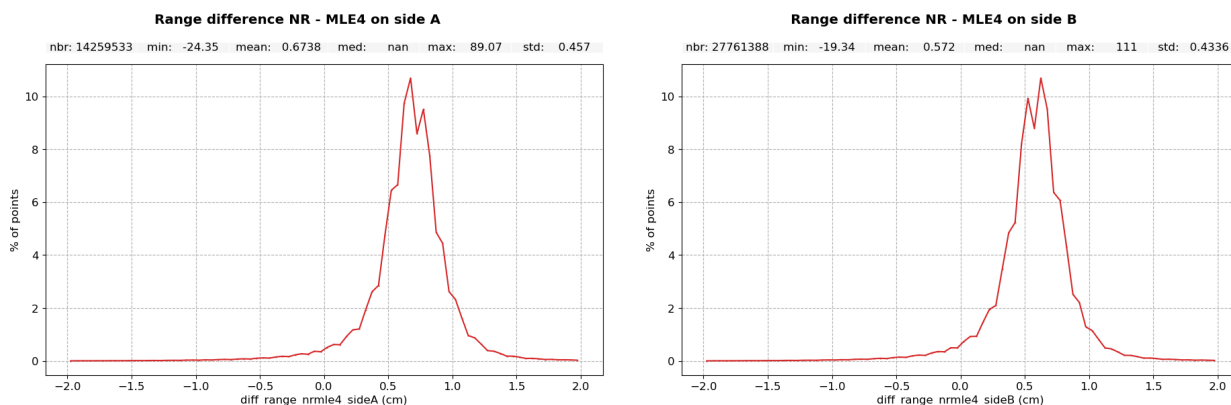
Figure 17 – Distributions of Sentinel-6 MF F08 NR - MLE4 range difference for side A ( left ) and side B ( right ).
