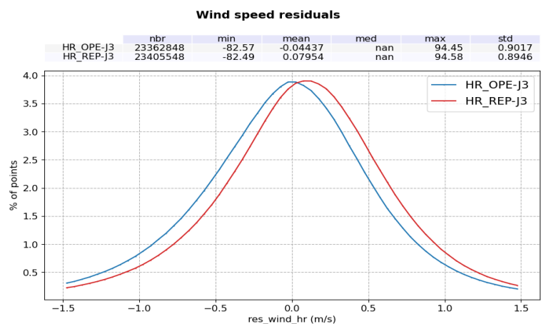
Figure 93 – Histogram of altimeter wind speed difference: Sentinel-6 MF HR minus Jason-3. Computed over the complete tandem period for operational (blue) and reprocessed (red) datasets.
