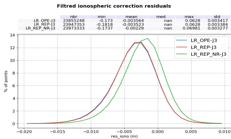
Figure 108 – Histogram of Filtered Altimeter Ionosphere correction difference: Sentinel-6 MF LR minus Jason-3. Computed over the complete tandem period for operational MLE4 (blue), reprocessed MLE4 (red) and NR (green).
