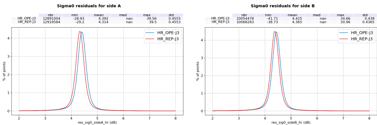
Figure 90 – Histogram of Ku-band backscatter coefficient difference: Sentinel-6 MF HR minus Jason-3. Computed over POS-4 side A (left) and side B (right) periods, for operational (blue) and reprocessed (red) datasets.
