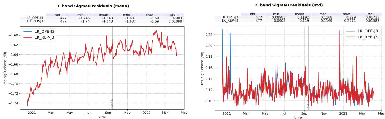
Figure 103 – Time monitoring of C-band backscatter coefficient difference: Sentinel-6 MF LR minus Jason-3. Mean per day (left) and standard deviation per day (right) computed over the complete tandem period, for the operational (blue) and reprocessed (red) datasets.
