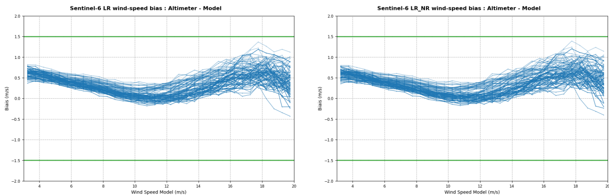
Figure 136 – Difference between Altimeter LR wind speed and model wind speed function of model wind speed, in m/s for MLE4 ( left ) and NR ( right ). Computed for all cycles (right, darker curves correspond to more recent cycles). Green lines represent requirement limits.
