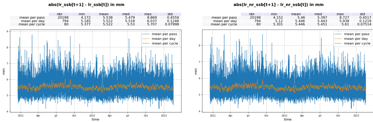
Figure 128 – Absolute value of consecutive LR sea state bias measurement for LR MLE4 (left) and NR (right). Mean per pass (blue), mean per day (orange) and mean per cycle (green).
