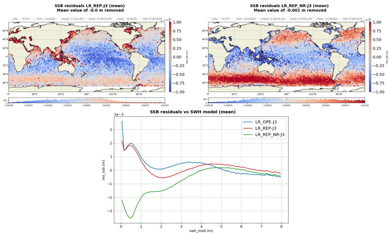
Figure 86 – Ku-band SSB difference: Sentinel-6 MF LR minus Jason-3 computed over the complete tandem period. Gridded map for reprocessed MLE4 ( left ) and NR ( right ) and difference function of ERA 5 model SWH ( bottom ).
