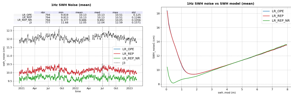
Figure 11 – 1Hz noise for LR operational (blue) and reprocessed (red for MLE4, green for NR) SWH, as a function of time ( left ) and ERA 5 model SWH ( right ).
