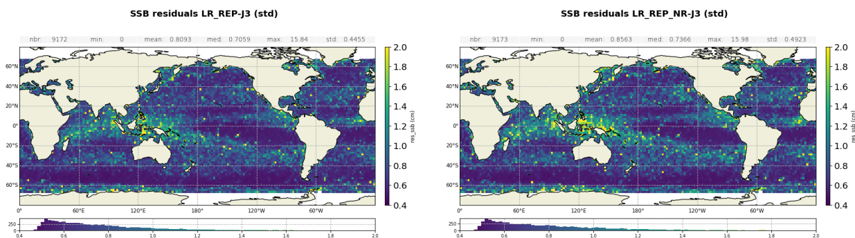
Figure 129 – Standard deviation gridded map of Ku-band SSB difference: Sentinel-6 MF LR minus Jason-3 computed over the complete tandem period for MLE4 (left) and NR (right).
