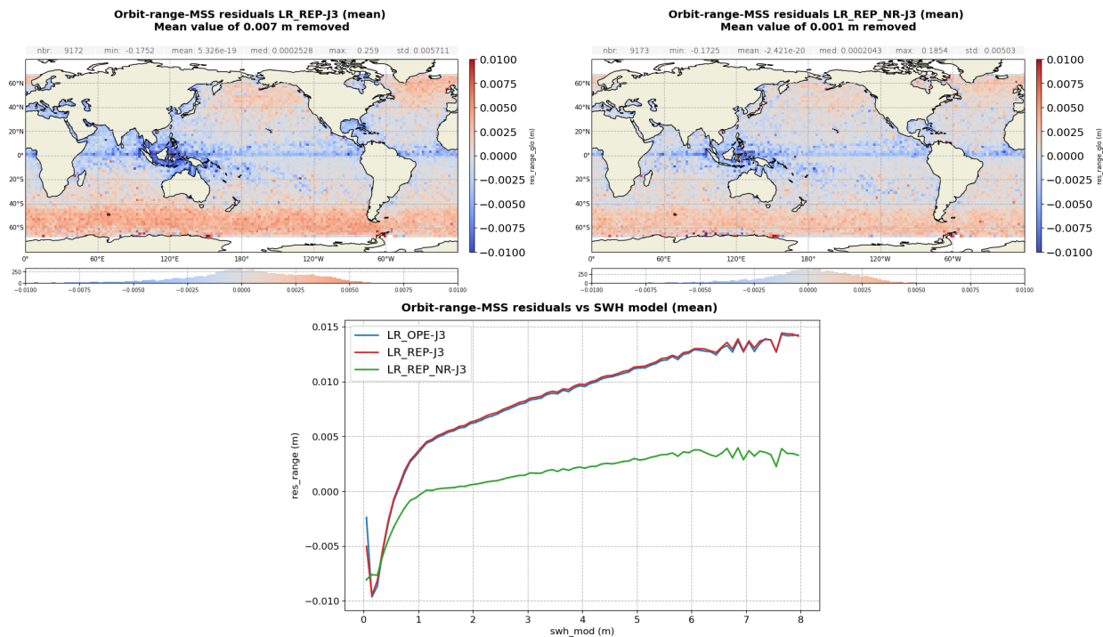
Figure 77 – Orbit - Ku-band range - MSS difference: Sentinel-6 MF LR minus Jason-3 computed over the complete tandem period. Gridded maps for reprocessed MLE4 ( left ) and NR ( right ) and difference function of ERA 5 model SWH ( bottom ).
