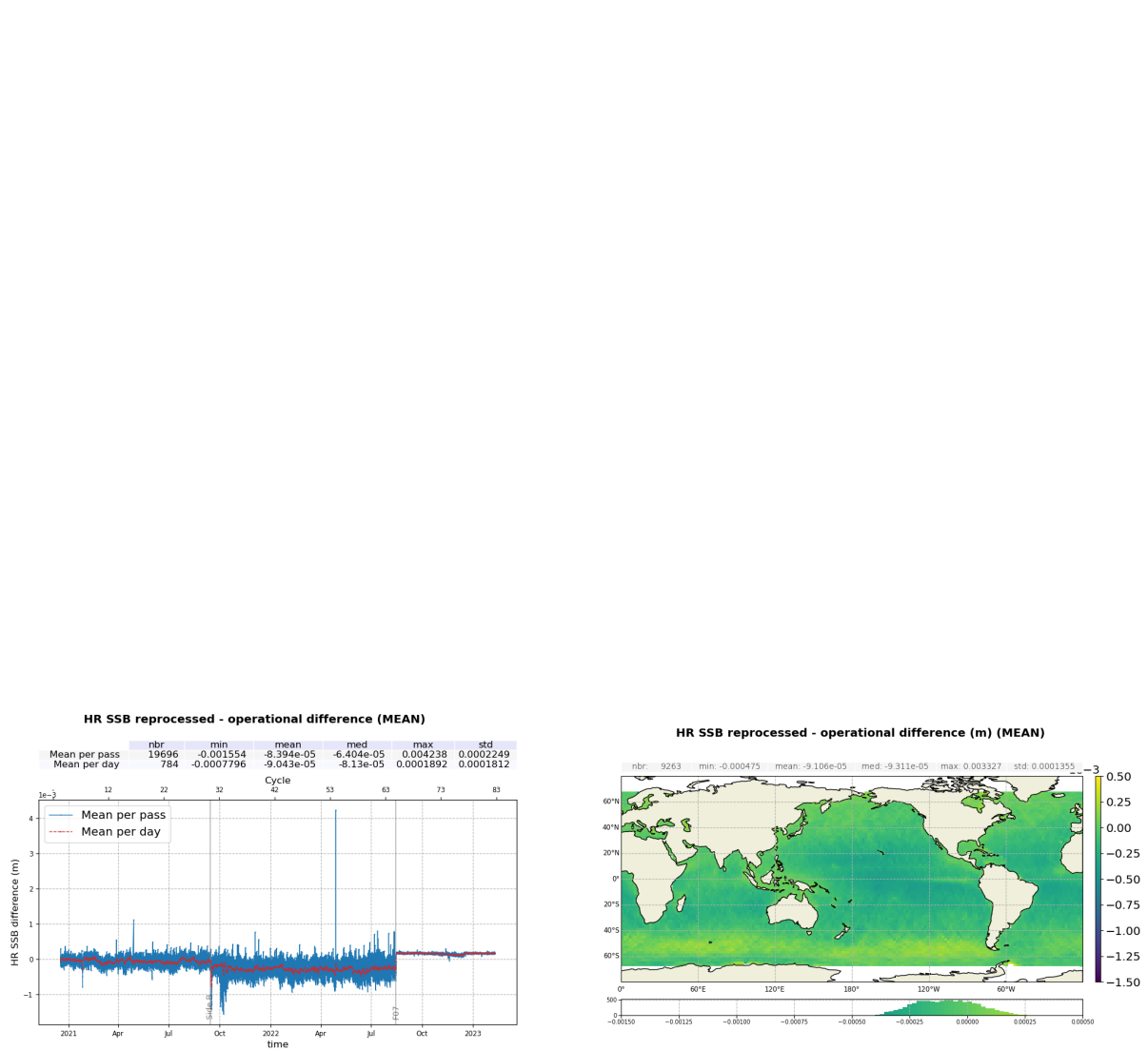
Figure 41 – Map ( right ) and monitoring ( left ) of the HR operational - reprocessed SSB difference per day (red) and per pass (blue).
