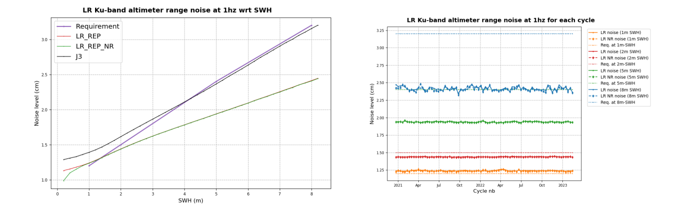
Figure 123 – 1 Hz noise of LR Ku-band altimeter range. Left panel: noise function of SWH for Sentinel-6 MF LR MLE4 (blue for MLE4, green for NR) and Jason-3 (black); the purple line represents the requirement thresholds. Right panel : noise level computed for each cycle and at 1, 2, 5 and 8 m-wave (solid lines for MLE4, dashed lines for NR) and the corresponding requirement levels (dotted lines).
