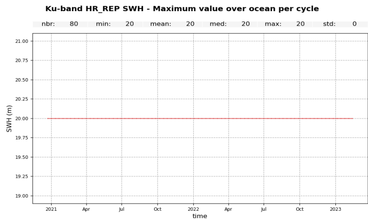
Figure 142 – Maximum value of Sentinel-6 MF HR SWH per cycle.
