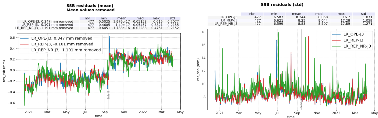
Figure 85 – Time monitoring of Ku-band SSB difference: Sentinel-6 MF LR minus Jason-3. Mean per day (left) and standard deviation per day (right) computed over the complete tandem period for operational MLE4 (blue), reprocessed MLE4 (red) and NR (green). Means have been centred on 0 for better visibility.
