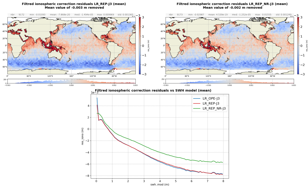
Figure 110 – Filtered Altimeter Ionosphere correction difference: Sentinel-6 MF LR minus Jason-3 computed over the complete tandem period. Gridded map for reprocessed MLE4 ( left ) and NR ( right ) and difference function of ERA 5 model SWH ( bottom ).
