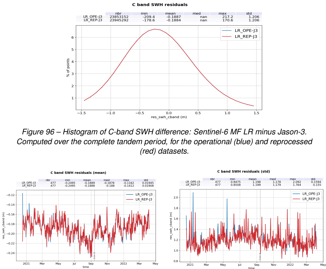
Figure 97 – Time monitoring of C-band SWH difference: Sentinel-6 MF LR minus Jason-3. Mean per day (left) and standard deviation per day (right) computed over the complete tandem period, for the operational (blue) and reprocessed (red) datasets.
