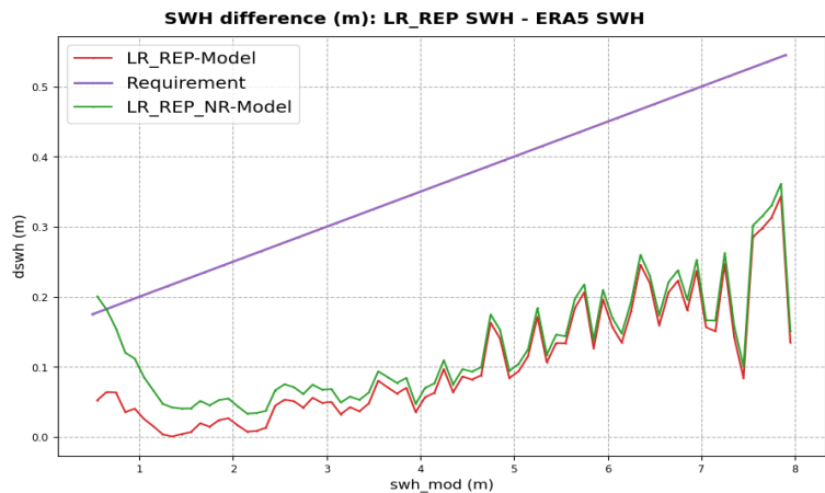
Figure 134 – SWH difference between Sentinel-6 MF LR data and ERA-5 SWH, plotted function of ERA-5 SWH for MLE4 (red) and NR (green). Computed over Sentinel-6 MF cycle 40. Purple lines represent requirement limits. Results are identical for all cycles.
