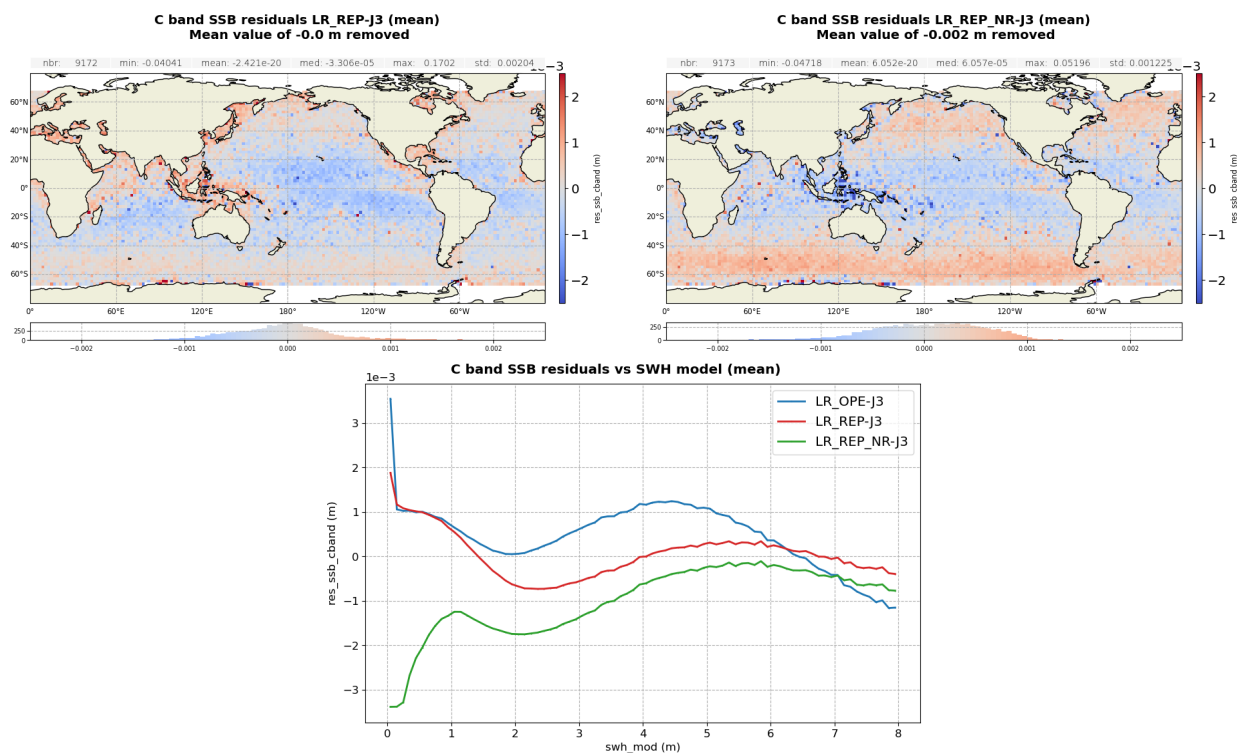
Figure 107 – C-band SSB difference: Sentinel-6 MF LR minus Jason-3 computed over the complete tandem period. Gridded map for reprocessed MLE4 ( left ) and NR ( right ) and difference function of ERA 5 model SWH ( bottom ).
