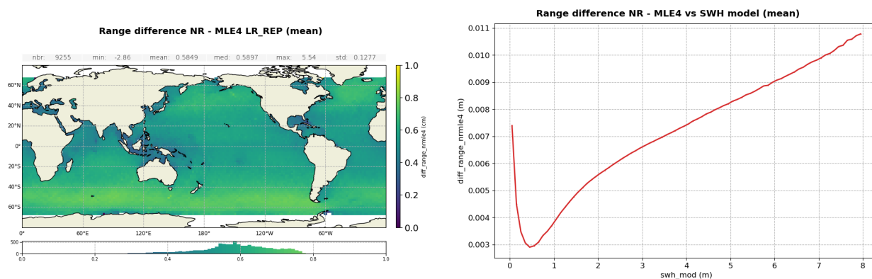
Figure 18 – Map ( left ) and ERA 5 model SWH dependency ( right ) of the LR F08 NR - MLE4 range difference.
