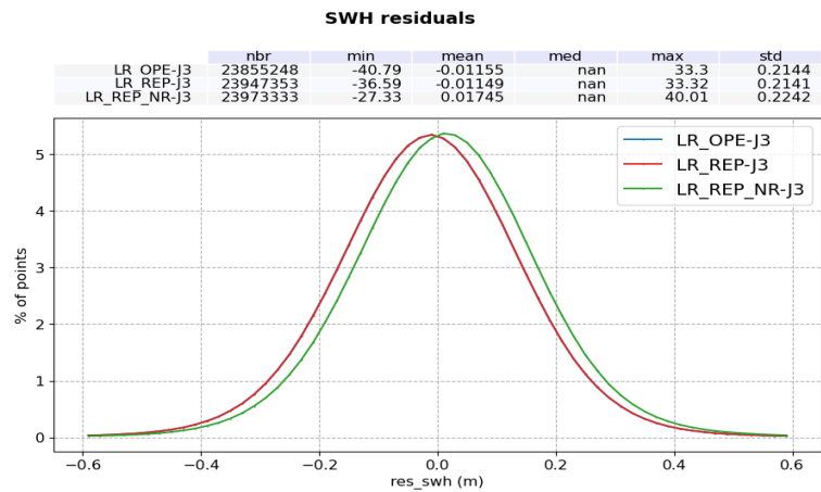
Figure 72 – Histogram of Ku-band SWH difference: Sentinel-6 MF LR minus Jason-3. Computed over the complete tandem period.
