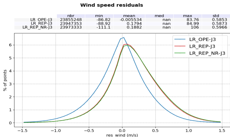
Figure 81 – Histogram of altimeter wind speed difference: Sentinel-6 MF LR minus Jason-3. Computed over the complete tandem period for operational MLE4 (blue), reprocessed MLE4 (red) and NR (green).
