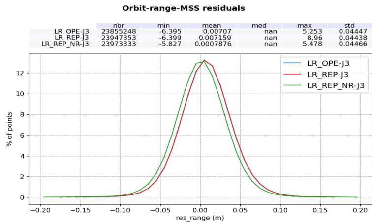
Figure 75 – Histogram of Orbit - Ku-band range - MSS difference : Sentinel-6 MF LR minus Jason-3. Computed over the complete tandem period.
