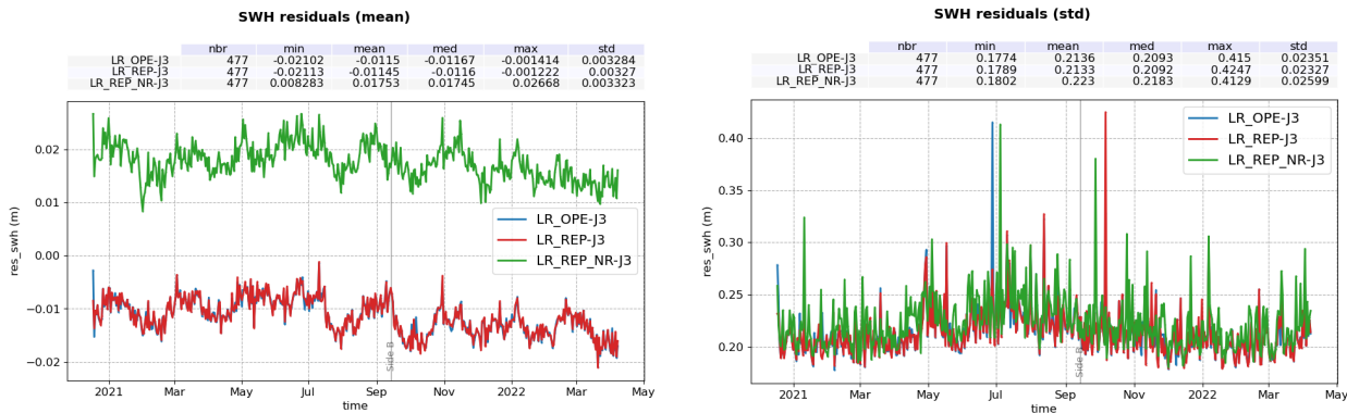
Figure 73 – Time monitoring of Ku-band SWH difference: Sentinel-6 MF LR minus Jason-3. Mean per day (left) and standard deviation per day (right) computed over the complete tandem period.
