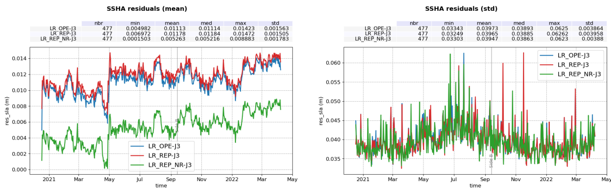
Figure 112 – Time monitoring of product SSHA difference: Sentinel-6 MF LR minus Jason-3. Mean ( left ) and standard deviation ( right ) per day computed over the complete tandem period for operational MLE4 (blue), reprocessed MLE4 (red) and NR (green).
