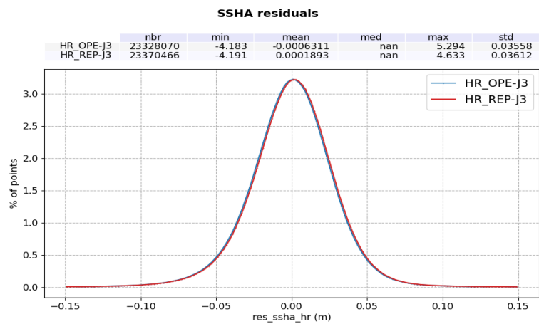
Figure 115 – Histogram of product SSHA difference: Sentinel-6 MF HR minus Jason-3. Computed over the complete tandem period for operational (blue) and reprocessed (red) datasets.
