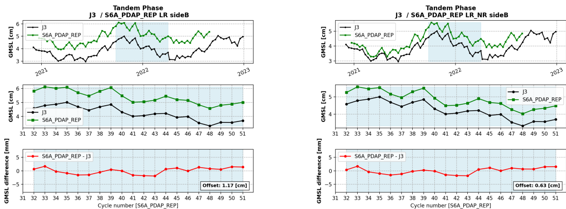
Figure 120 – Jason-3 (black) and Sentinel-6 MF (green) GMSL over the side B (top panel), the tandem phase (middle panel) and their differences over the side B tandem phase (bottom panel), for Sentinel-6 MF reprocessed dataset, LR MLE4 on the left and LR NR on the right.
