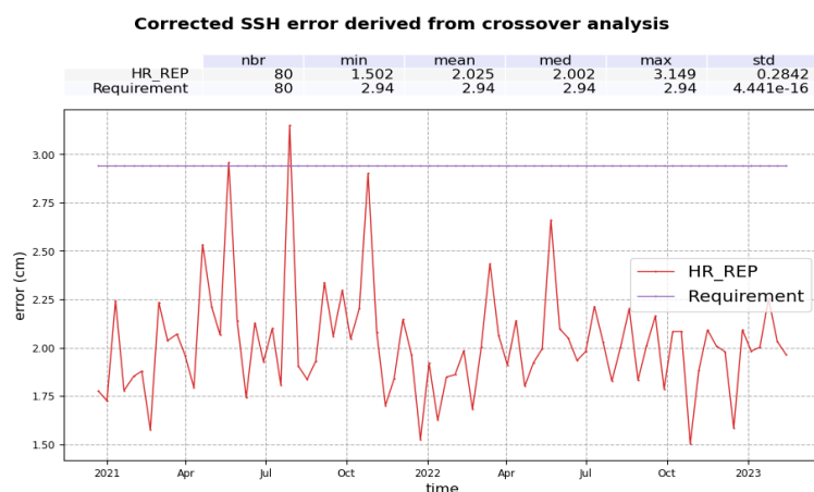
Figure 140 – Corrected HR SSH error derived from crossover analysis with a selection over Pacific patch (latitude in [-24.5^{\circ}\text{N}; -3^{\circ}\text{N}] and longitude in [220^{\circ}\text{E}; 246^{\circ}\text{E}] ), in cm. The error equals to the standard deviation of the SSH difference divided by \sqrt{(2)} . Computed on a cyclic basis.
