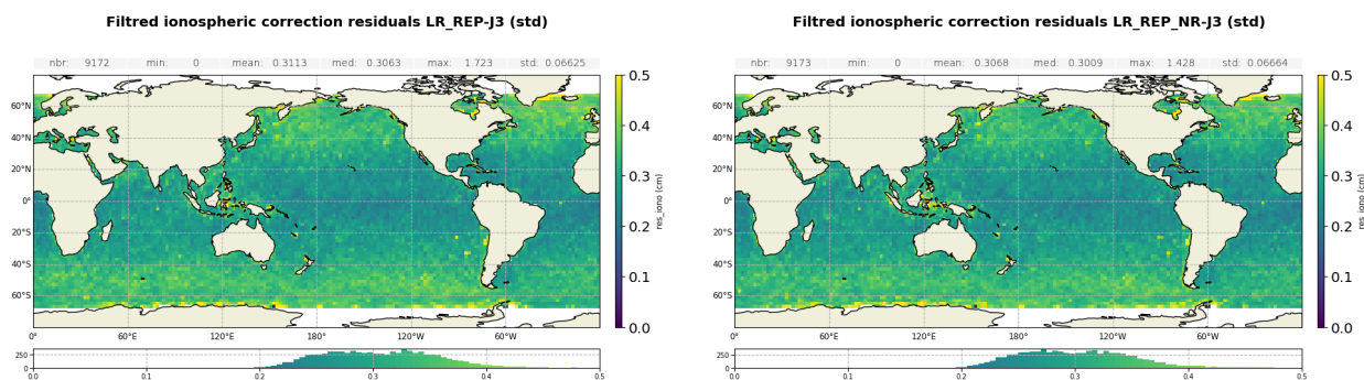
Figure 126 – Standard deviation gridded map of Altimeter Filtered Ionosphere correction Sentinel-6 MF-Jason-3 difference (cm) for MLE4 ( left ) and NR ( right ). Computed over the tandem phase.
