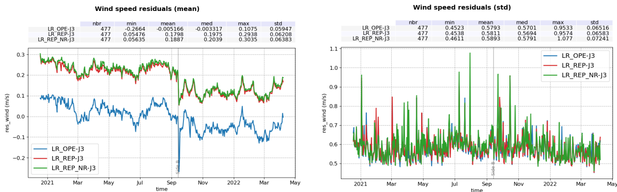
Figure 82 – Time monitoring of Ku-band wind speed difference: Sentinel-6 MF LR minus Jason-3. Mean per day ( left ) and standard deviation per day ( right ) computed over the complete tandem period for operational MLE4 (blue), reprocessed MLE4 (red) and NR (green).
