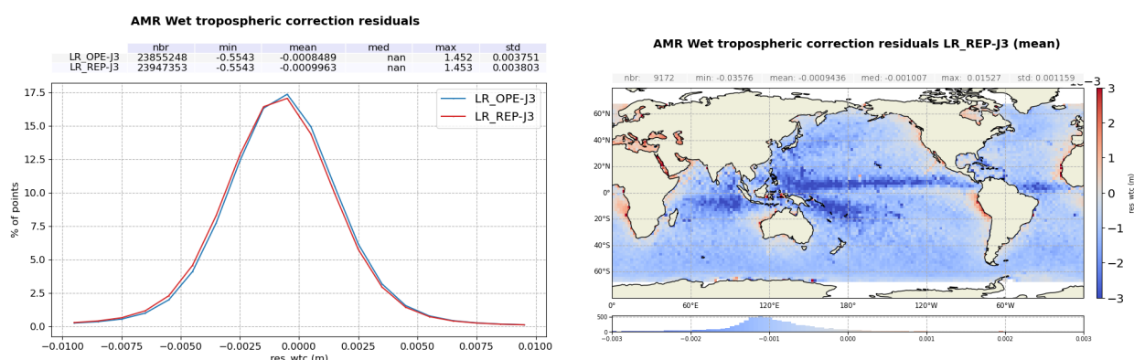
Figure 70 – Radiometer WTC difference : Sentinel-6 MF AMR-C/HRMR minus Jason-3 AMR. Histogram ( left ) and gridded map ( right ) computed over the complete tandem period.
