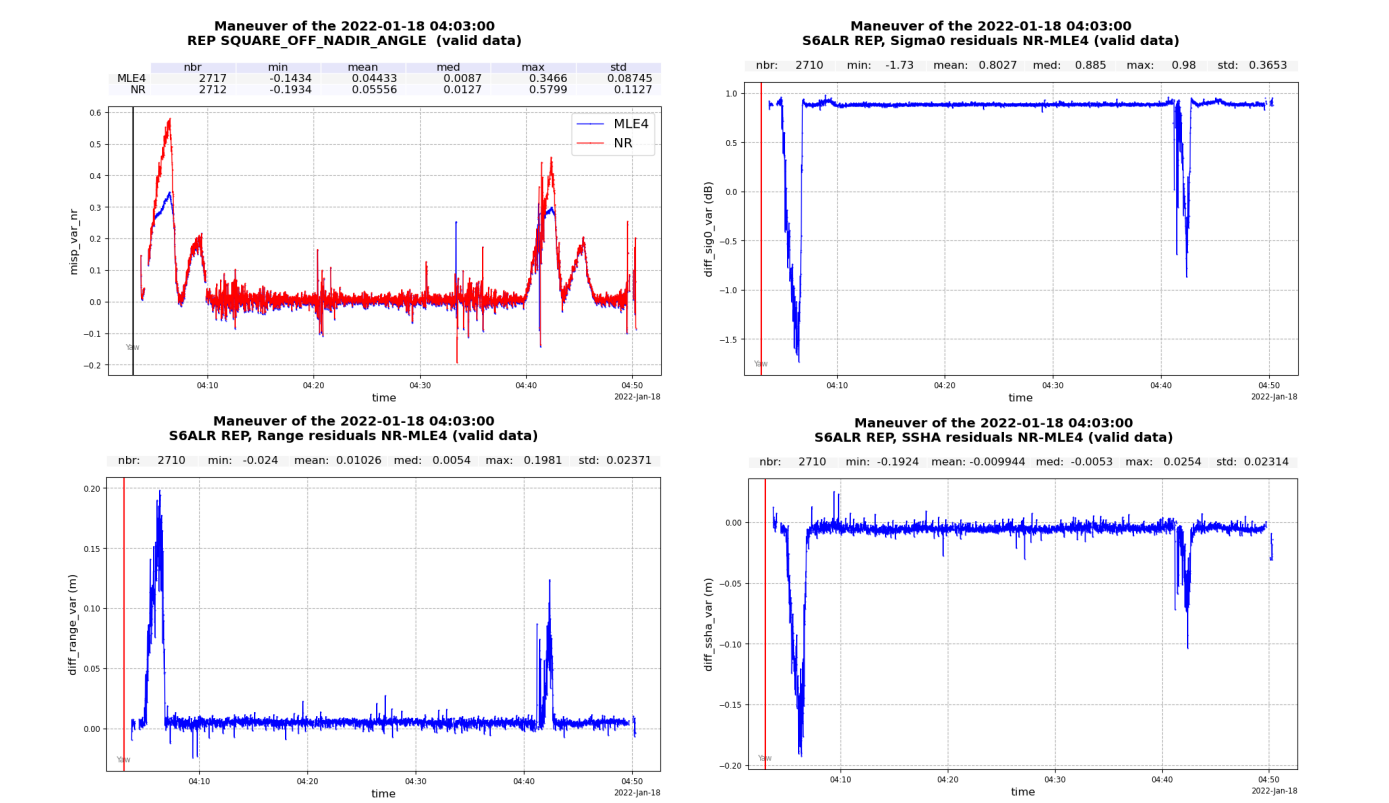
Figure 53 – Sentinel-6 MF along-track reprocessed MLE4 (blue) and NR (red) square off-nadir angle ( top left ) and reprocessed NR - MLE4 sigma0 ( top right ), range ( bottom left ) and SSHA ( bottom right ) for cycle 44 pass 4.
