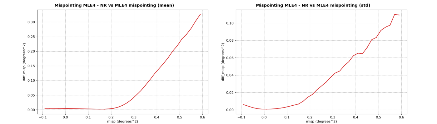
Figure 51 – Sentinel-6 MF LR reprocessed MLE4 - NR square off-nadir angle differences as a function of the reprocessed MLE4 square off-nadir angle. Left : mean, right : standard deviation.
