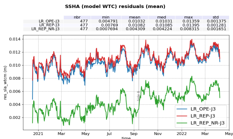
Figure 113 – Time monitoring of product SSHA with model WTC difference: Sentinel-6 MF LR minus Jason-3. Mean per day computed over the complete tandem period for operational MLE4 (blue), reprocessed MLE4 (red) and NR (green).
