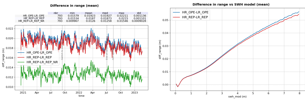
Figure 20 – Time monitoring (left) and ERA 5 model SWH dependency (right) of Sentinel-6 MF Ku-band Range difference : HR - LR, before reprocessing (blue) and after reprocessing (red with LR MLE4 and green for LR NR)
