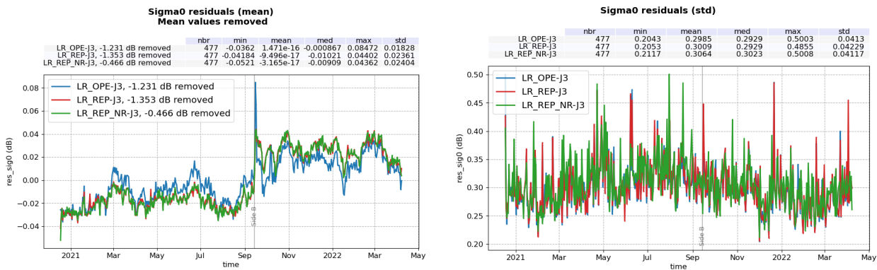
Figure 79 – Time monitoring of Ku-band backscatter coefficient difference: Sentinel-6 MF LR minus Jason-3. Mean per day (left) and standard deviation per day (right) computed over the complete tandem period for operation MLE4 (blue), reprocessed MLE4 (red) and NR (green).
