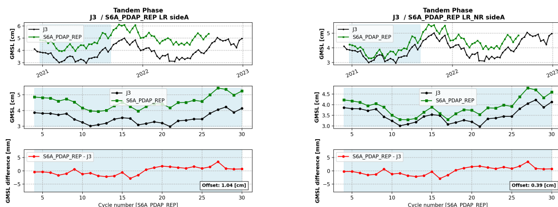
Figure 118 – Jason-3 (black) and Sentinel-6 MF (green) GMSL over the side A (top panel), the tandem phase (middle panel) and their differences over the side A tandem phase (bottom panel), for Sentinel-6 MF reprocessed dataset, LR MLE4 on the left and LR NR on the right.
