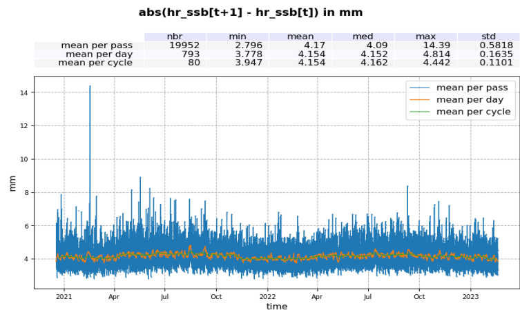
Figure 138 – Absolute value of consecutive HR sea state bias measurement. Mean per pass (blue), mean per day (orange) and mean per cycle (green).
