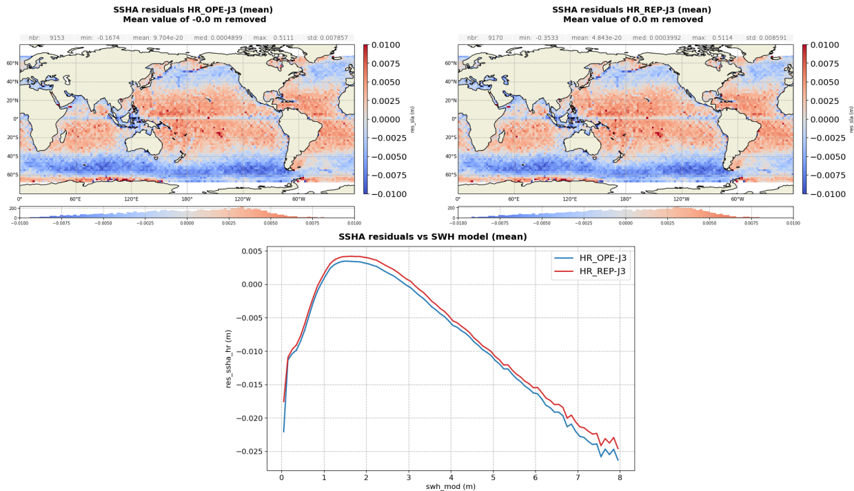
Figure 117 – SSHA difference: Sentinel-6 MF HR minus Jason-3 computed over the complete tandem period. Gridded map for operational ( left ) and reprocessed ( right ) datasets and difference function of ERA 5 model SWH ( bottom ).
