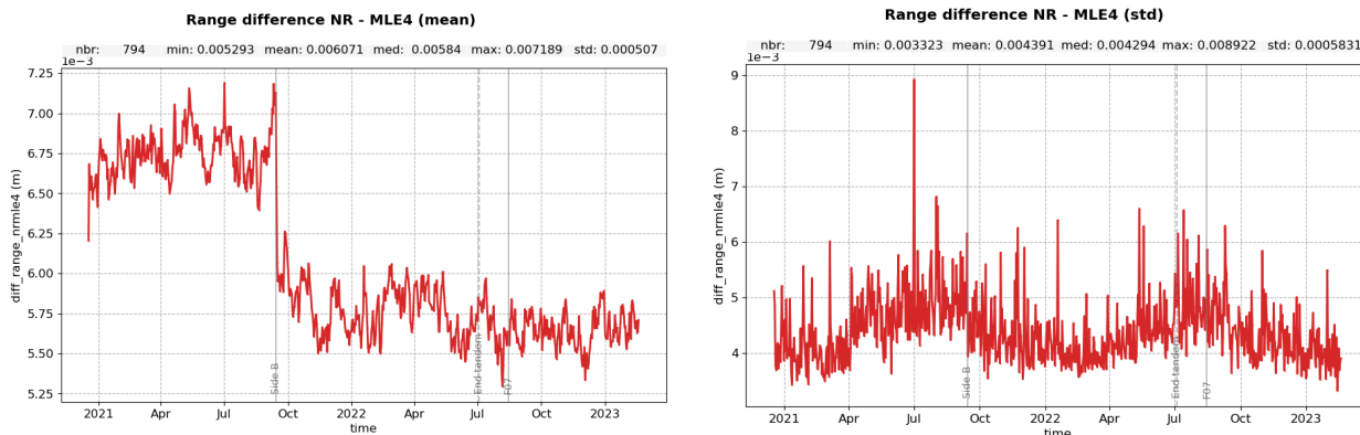
Figure 16 – Time monitoring of Sentinel-6 MF F08 NR - MLE4 range difference per day, for the mean ( left ) and the standard deviation ( right ).
