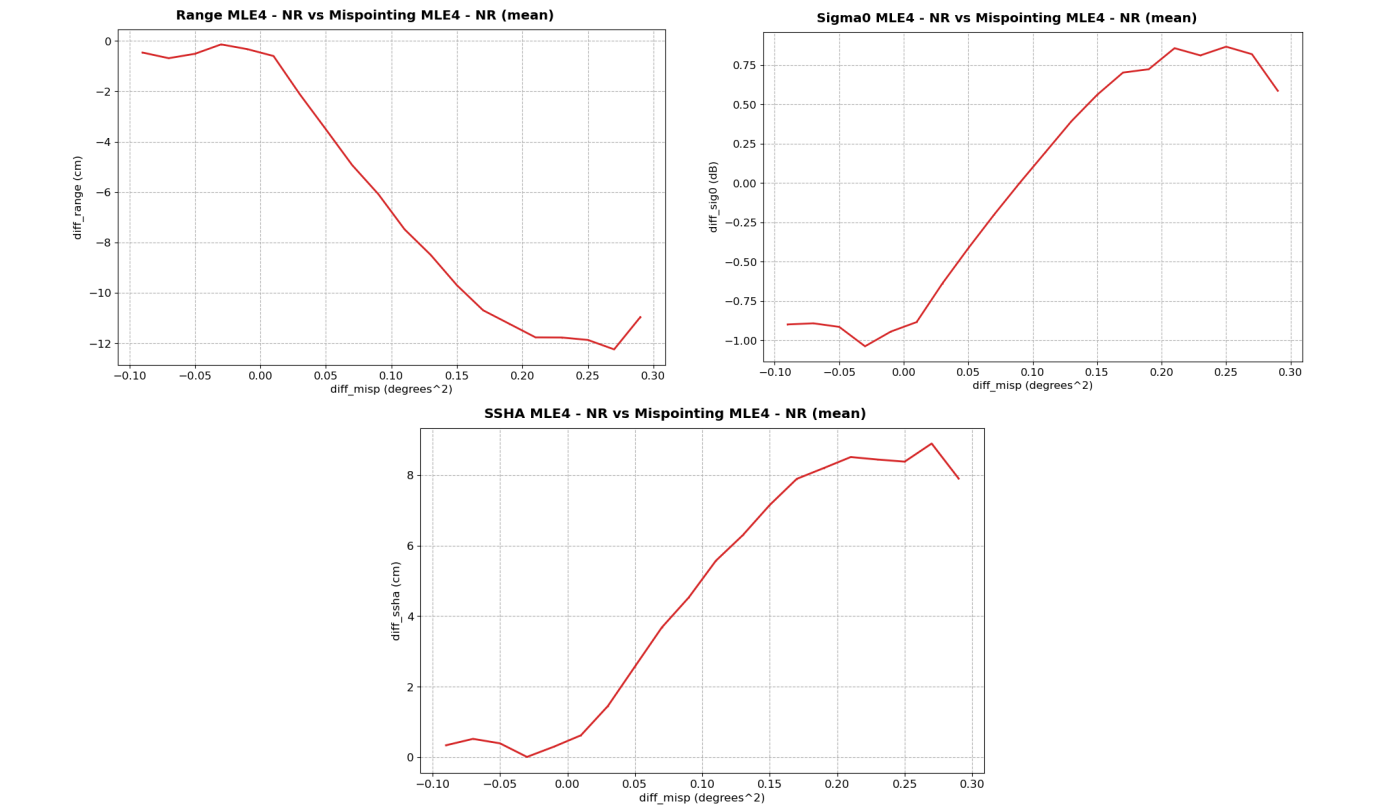
Figure 52 – Sentinel-6 MF LR reprocessed MLE4 - NR range ( left ), sigma0 ( right ) and SSHA ( bottom ) mean differences as a function of the reprocessed MLE4 - NR square off-nadir angle differences.
