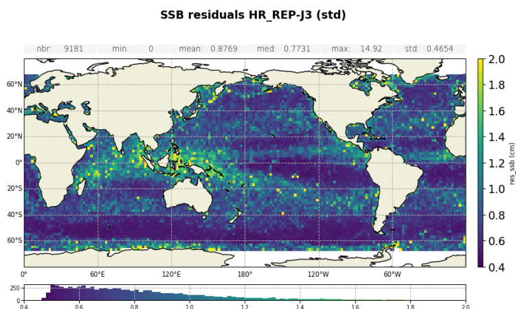
Figure 139 – Standard deviation gridded map of Ku-band SSB difference: Sentinel-6 MF HR minus Jason-3 computed over the complete tandem period.
