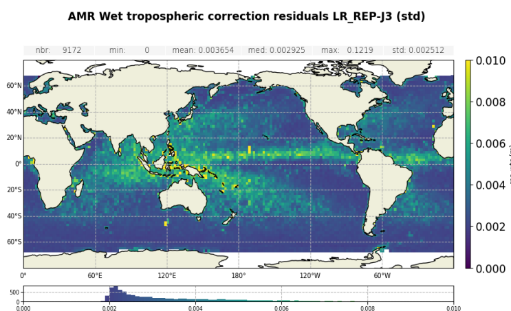
Figure 132 – STD gridded map of AMR WTC difference: Sentinel-6 MF LR minus Jason-3, in m. Computed over cycles 4 to 51.
