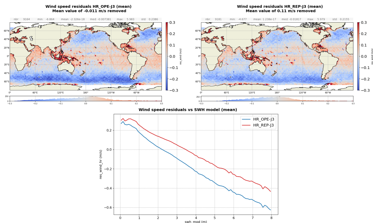
Figure 95 – Altimeter wind speed difference: Sentinel-6 MF HR minus Jason-3 computed over the complete tandem period in m/s. Gridded map for operational ( left ) and reprocessed ( right ) datasets and difference function of ERA 5 model SWH ( bottom ).
