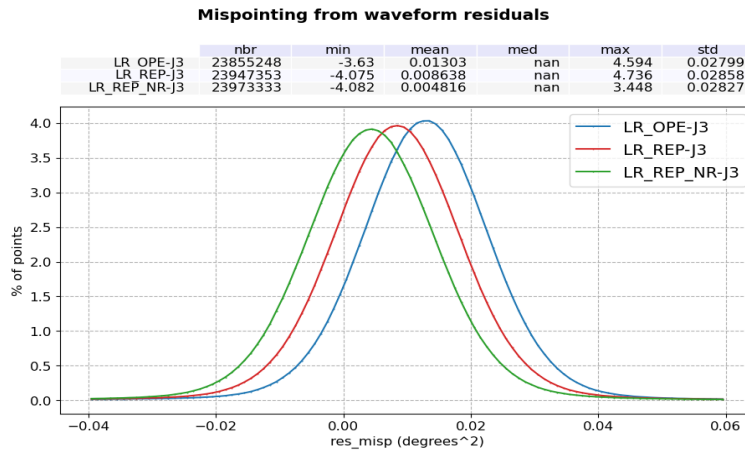
Figure 87 – Histogram of mispointing difference: Sentinel-6 MF LR minus Jason-3. Computed over the complete tandem period for operational MLE4 (blue), reprocessed MLE4 (red) and NR (green).
