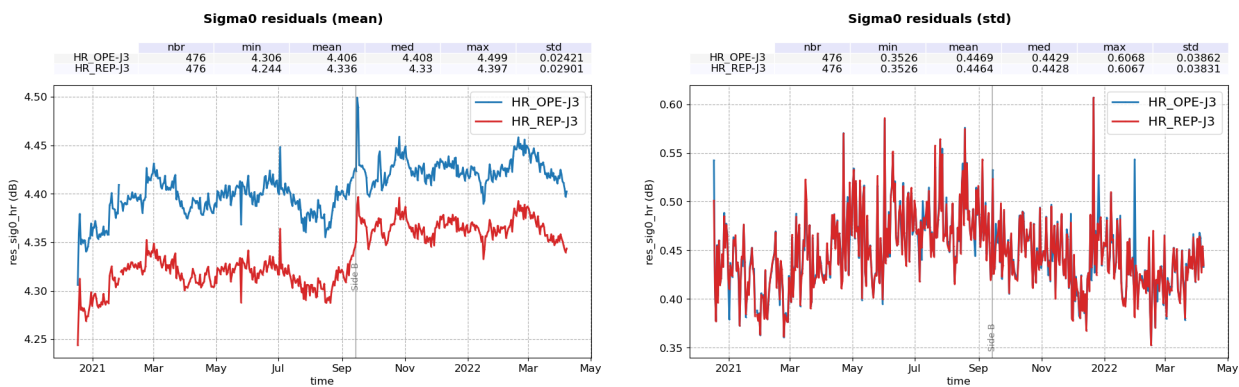
Figure 91 – Time monitoring of Ku-band backscatter coefficient difference: Sentinel-6 MF HR minus Jason-3. Mean per day (left) and standard deviation per day (right) computed over the complete tandem period for operational (blue) and reprocessed (red) datasets.
