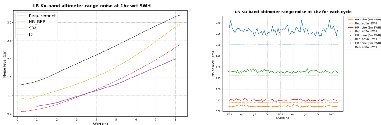
Figure 137 – 1 Hz noise of HR Ku-band altimeter range, in cm. Left panel: noise function of SWH in m for Sentinel-6 MF HR and Jason-3; the purple line represents the requirement thresholds. Right panel : noise level computed for each cycle and at 1, 2, 5 and 8 m-wave (solid lines) and the corresponding requirement levels (dashed lines).
