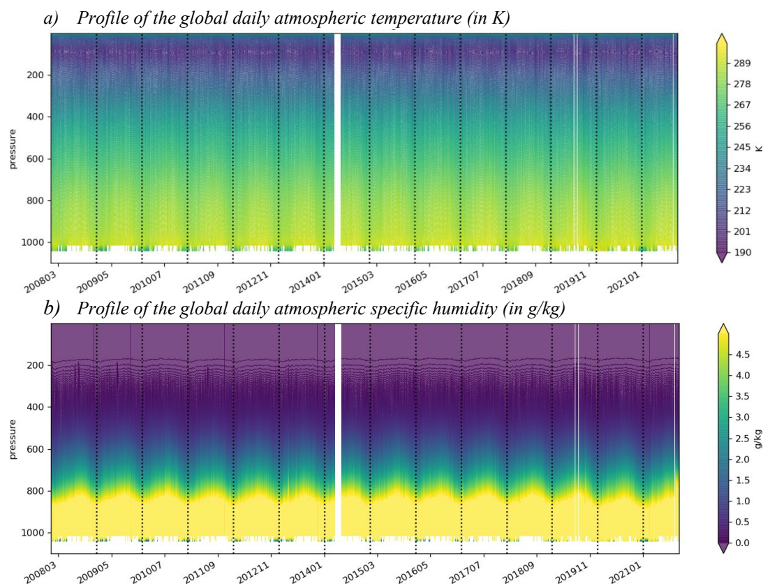
Figure 16: Hovmoeller plots of IASI-A temperature and specific humidity profiles, global daily average over the entire CDR range.
