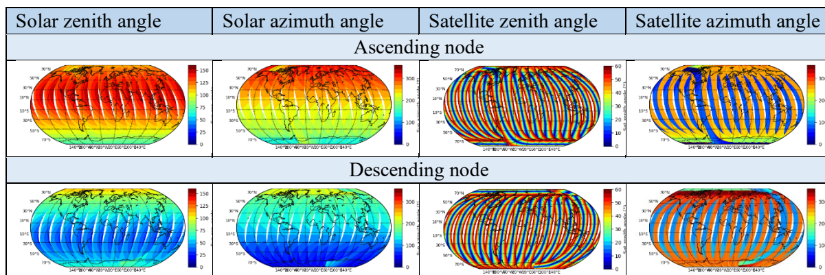
Figure 9: IASI-A solar and satellite zenith and azimuth angles for ascending and descending part of the orbit for the 1 st of January 2008.
