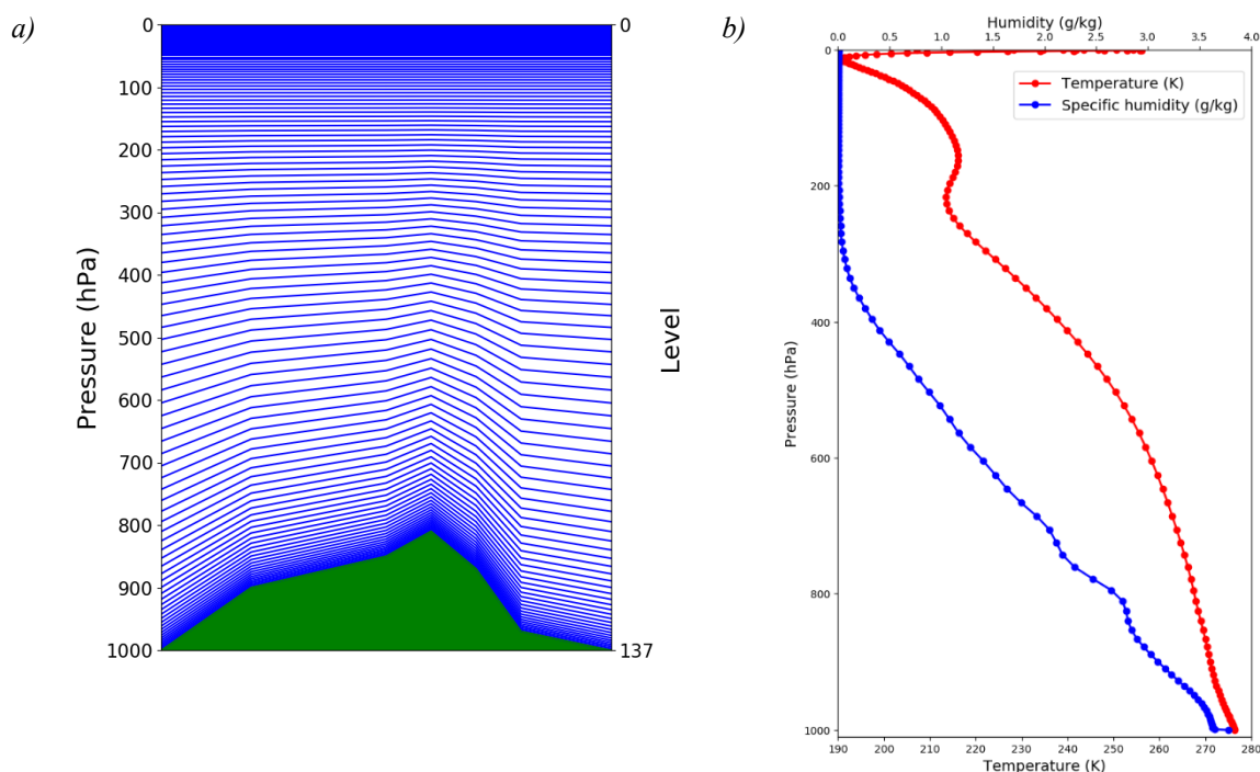
Figure 5: a) 137 hybrid sigma pressure levels and b) an example of a temperature and humidity atmospheric profile at one particular location.
