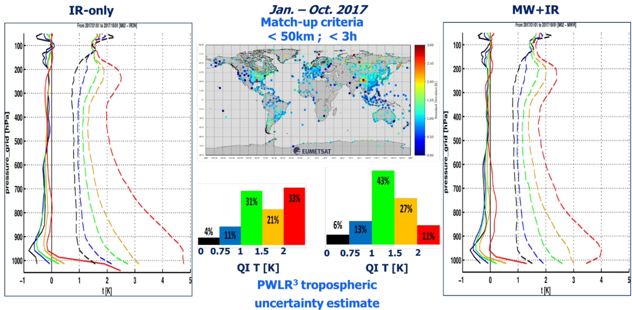
Figure 13: Temperature retrieval yield and precision in the IRON and MWIR modes stratified against the quality indicator (uncertainty estimate), assessed through 2017 with radiosonde measurement pre-processed in the NOAA Integrated Global Radiosonde Archive (IGRA). Solid lines are the bias and dash lines are the standard deviations. The colours represent data for several QI T ranges.
