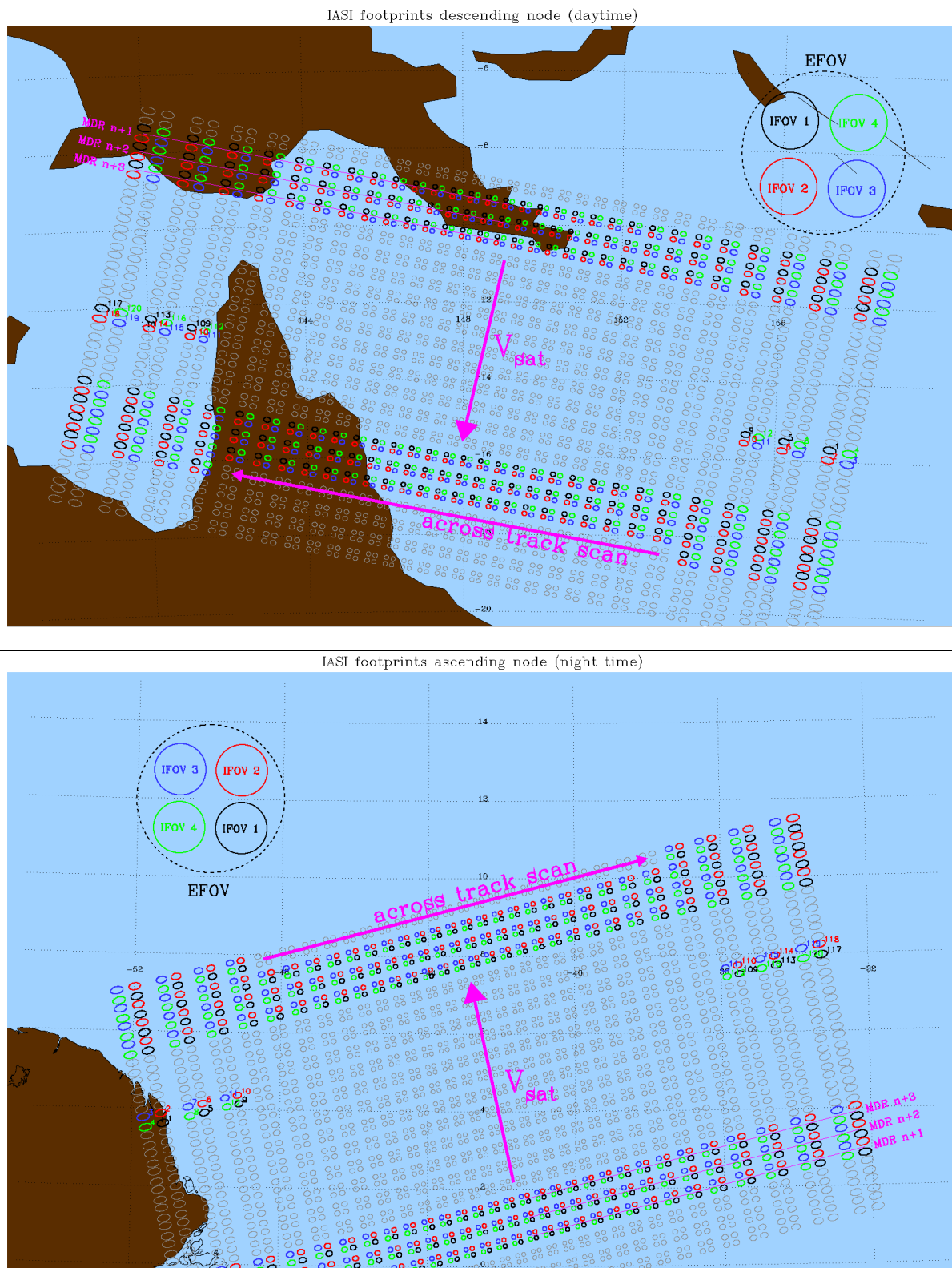
Figure 7: Example of location of IASI individual pixels for a descending orbit (top) and ascending orbit (bottom), note grey pixels are not coloured for clarity reasons, otherwise have the same content as the coloured pixels. Figures from: IASI_PW3_02_M02_20190126230859Z_20190126231154Z
