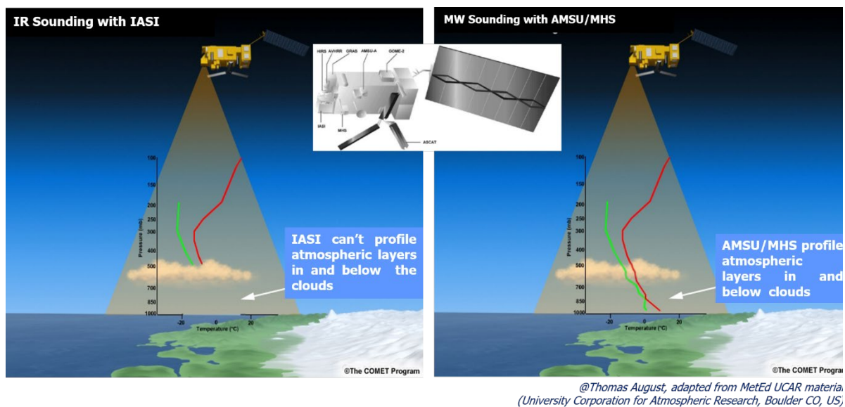
Figure 2: Synergy between infrared (IASI) and microwave (MHS and AMSU-A) instruments.
