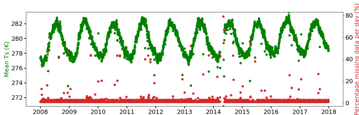
Figure 15: Example of a global IASI-A daily averaged surface temperature (K) in green. Red dots represent the percentage of missing data for a specific day. T_s is obtained using PWRL 3 .
