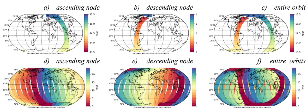
Figure 8: Example of the acquisition time (in hours) on the 1 st of January 2008.
