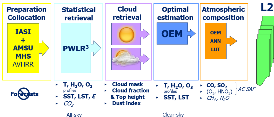
Figure 4: Overall picture of the operational EUMETSAT IASI level2 atmospheric product.
