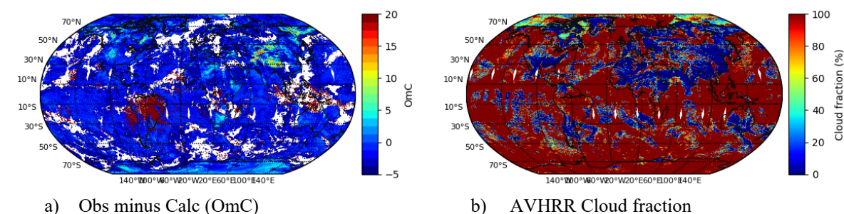
Figure 14: Example of daily maps of a) Observation minus Calculation and b) AVHRR Cloud fraction [IASI-A 2008/01/01]
