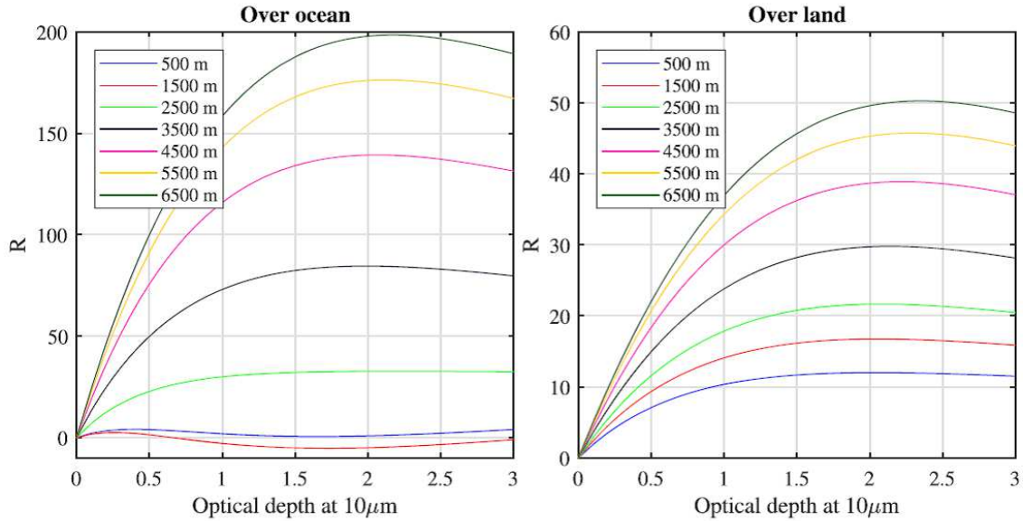
Figure 4.9: Dependence of the R value on altitude and dust OD for (left) an ocean and (right) a land scene.
