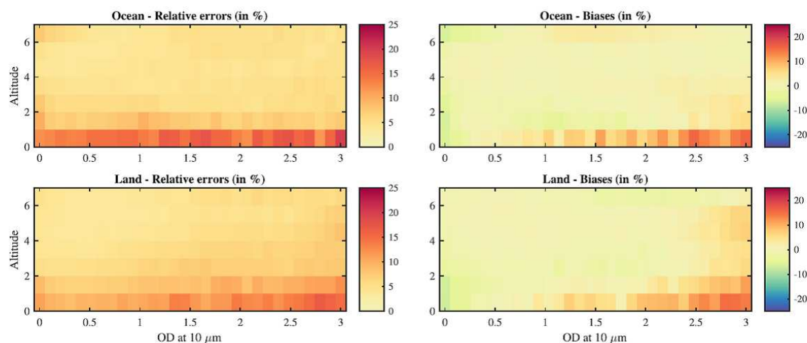
Figure 4.10: Performance of the NN on the training data set, in terms of relative errors (left panels) and biases (right panels) (colorscale shows percentage of relative errors/biases) as a function of OD (OD = optical depth) and altitude for ocean (top panels) and land (bottom panels) observations.
