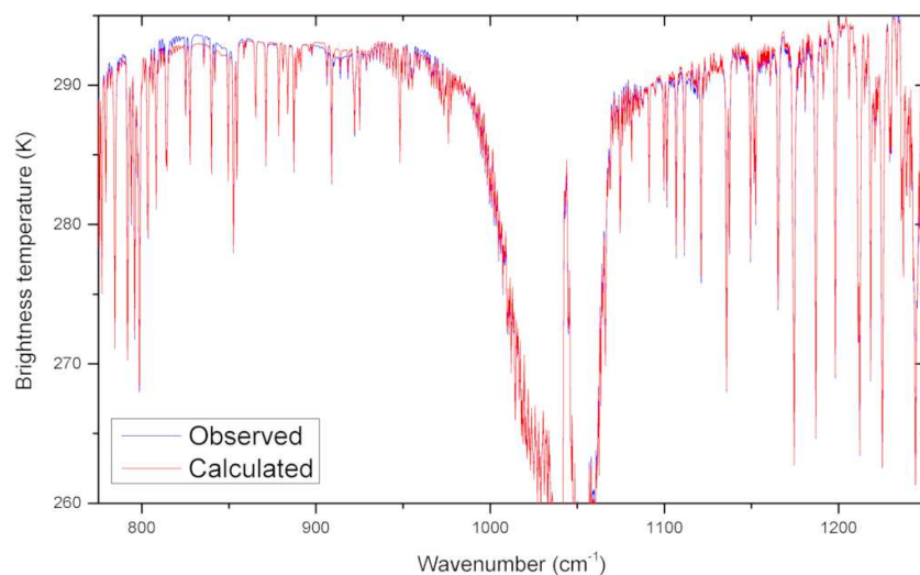
Figure 3.2: Mean observed and calculated spectrum with the Volz (1973) refractive indices.
