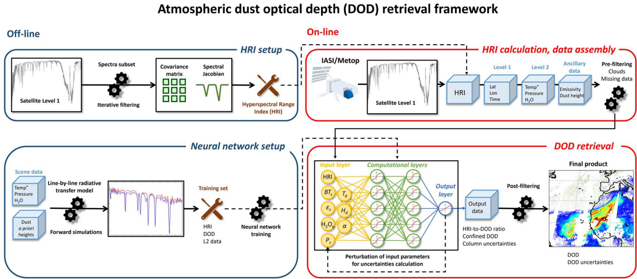
Figure 4.1: Flowchart showing the IASI atmospheric dust optical depth retrieval framework.
