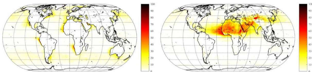
Figure 4.5: Percentage of cloud-free daytime observations in 2013 that are removed as they are potentially affected by temperature inversions (left panel), and the percentage of remaining observations detected as dust (right panel).
