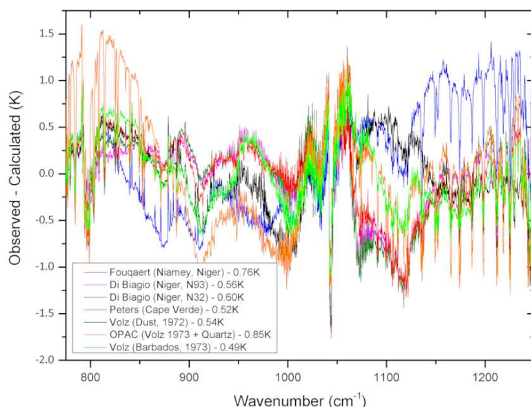
Figure 3.1: Retrieval residuals with 7 different refractive indices.
