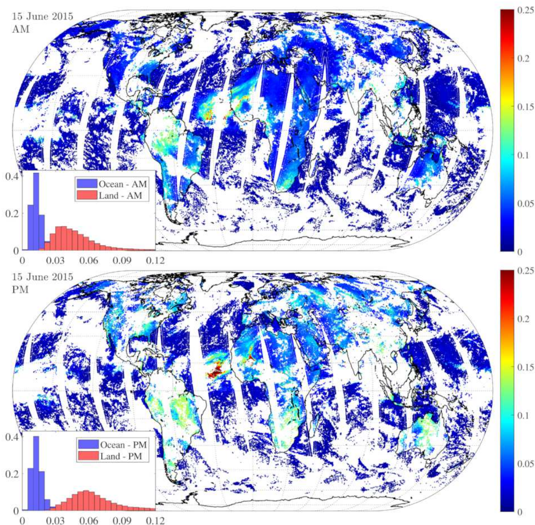
Figure 4.12: IASI-retrieved absolute OD uncertainties (unitless) for 15 June 2015 for the morning (top) and evening (bottom) overpass. The insets provide the probability histograms (frequency of each OD uncertainty values) of the global data.
