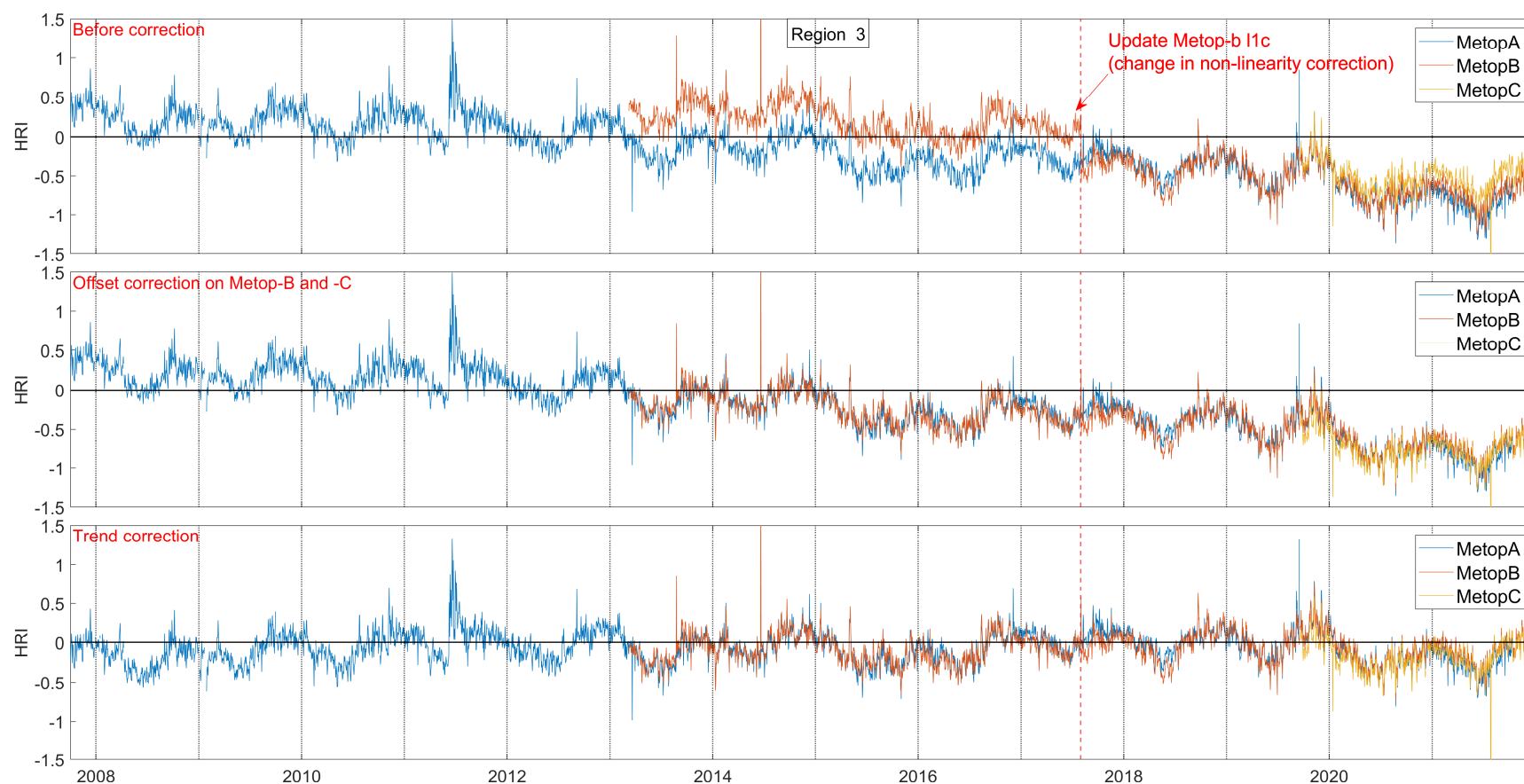
Figure 4.7: Example of the time series of R values for Metop-A, -B and -C for one region in the Indian Ocean (region 3 on Figure 4.6), (top) before the biases correction, (middle) after correction for the offset on Metop-B and Metop-C and (bottom) after correction for the trend bias.
