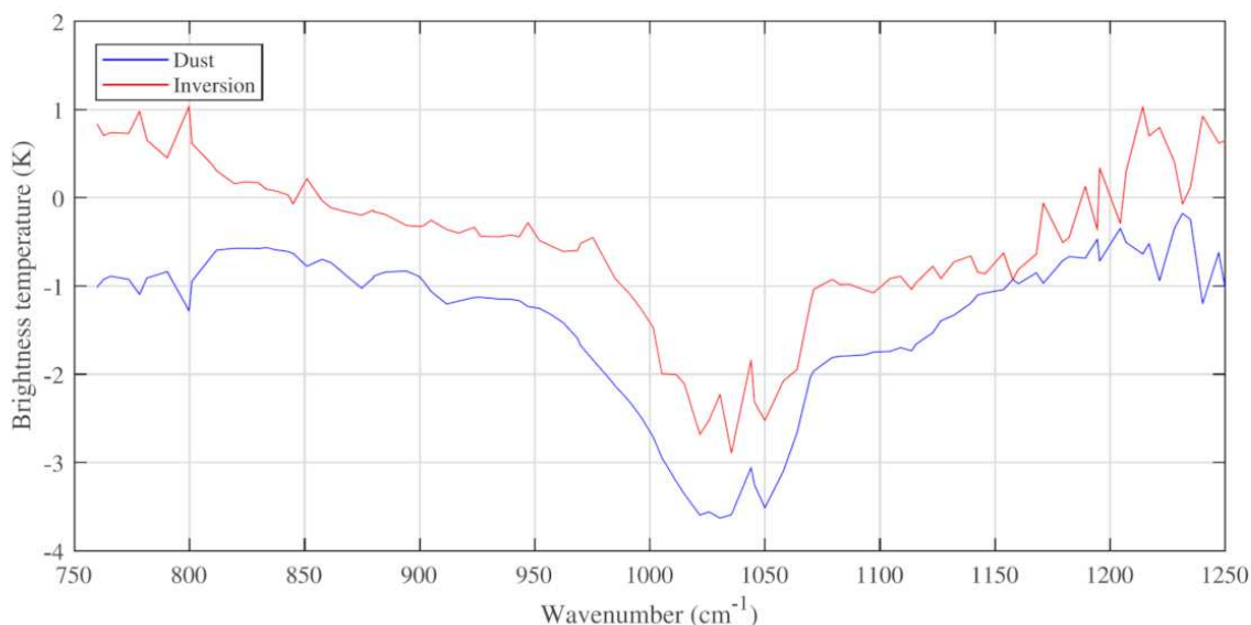
Figure 4.2: The IASI-derived Jacobian used for dust detection (blue) together with the Jacobian used for the removal of false detection due to large temperature inversions (red). The spectra shown have a reduced sampling of 100 channels.
