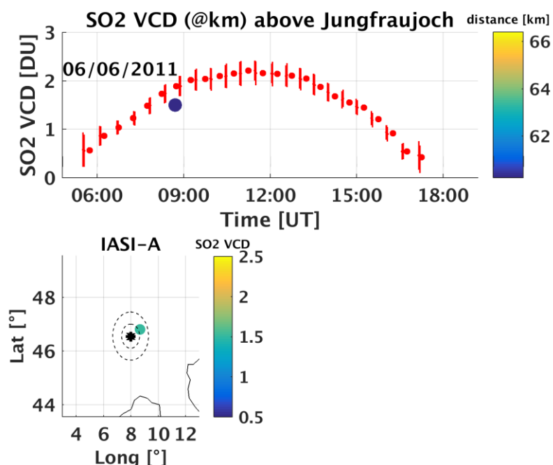
Figure 12. SO 2 VCD comparisons at Jungfraujoch on 6/6/2011 for the Grimsvotn eruption. The figure presents an upper panel, with the SO 2 VCD time-series from the zenith measurements (in red) and from IASI-A (SO 2 columns at the retrieved height, color-coded as a function of the station distance). The lower panels present the geographical distribution of the IASI-A SO 2 VCD around the station (circles at 50km and 100km are plotted in dotted lines).
