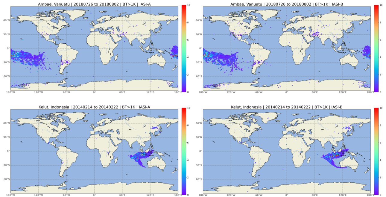
Figure 2. The IASI-A [left] and IASI-B [right] ΔBt > 1K SO 2 loads during the Ambae, 2018 eruption [upper] and the Kelut, 2014 eruption [lower].
